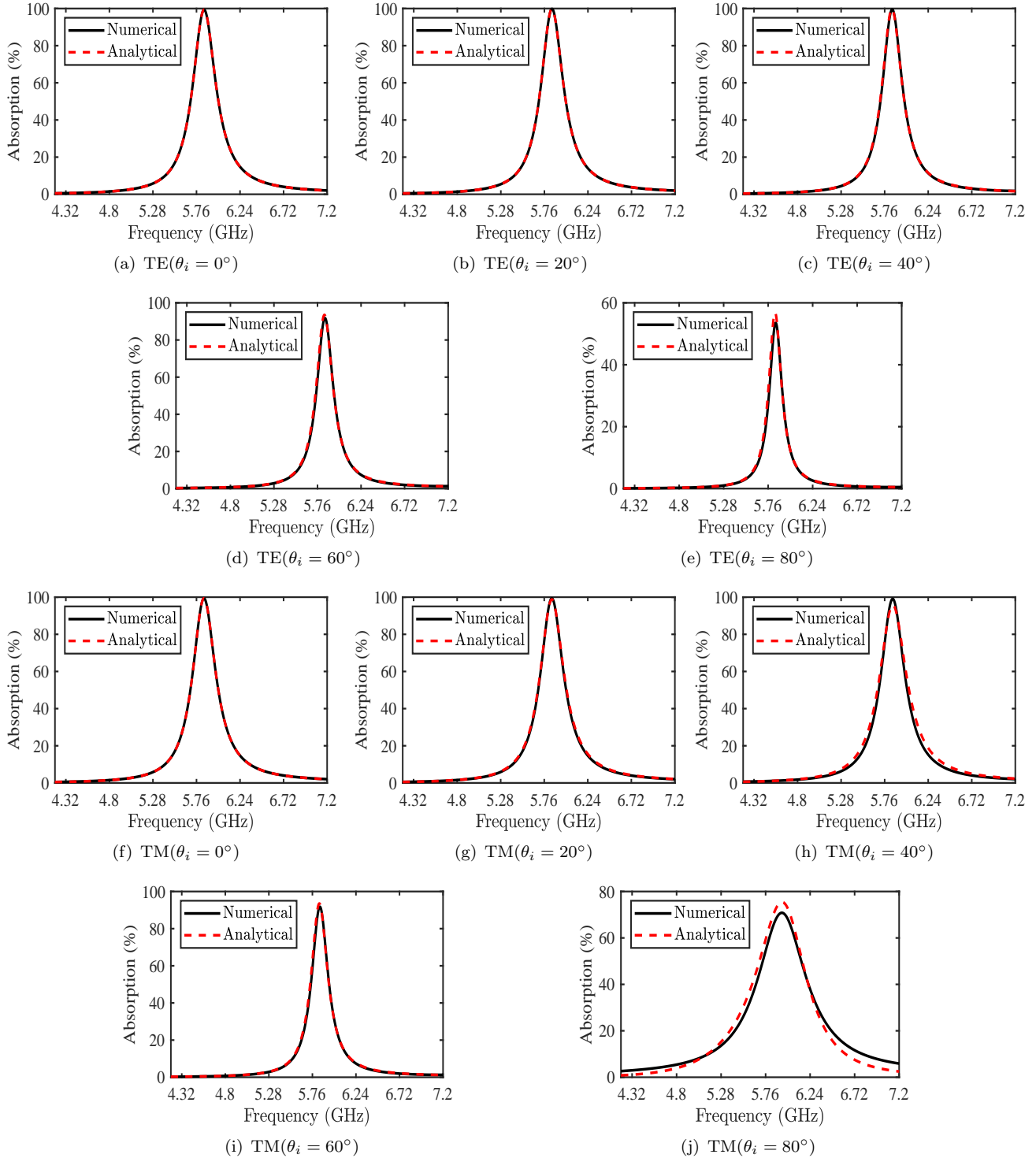
Figure 6. Comparison between numerically simulated and analytically calculated absorption curves for different values of the incidence angle \theta_i . (a),(b),(c),(d) and (e) Case of TE. (f),(g),(h),(i) and (j) Case of TM.
