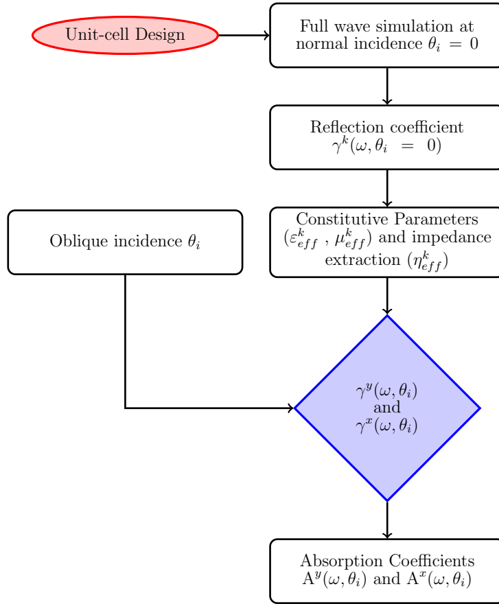
Figure 2. Step by step flowchart model for absorption estimation in oblique incidence from unit-cell response under normal incidence.
