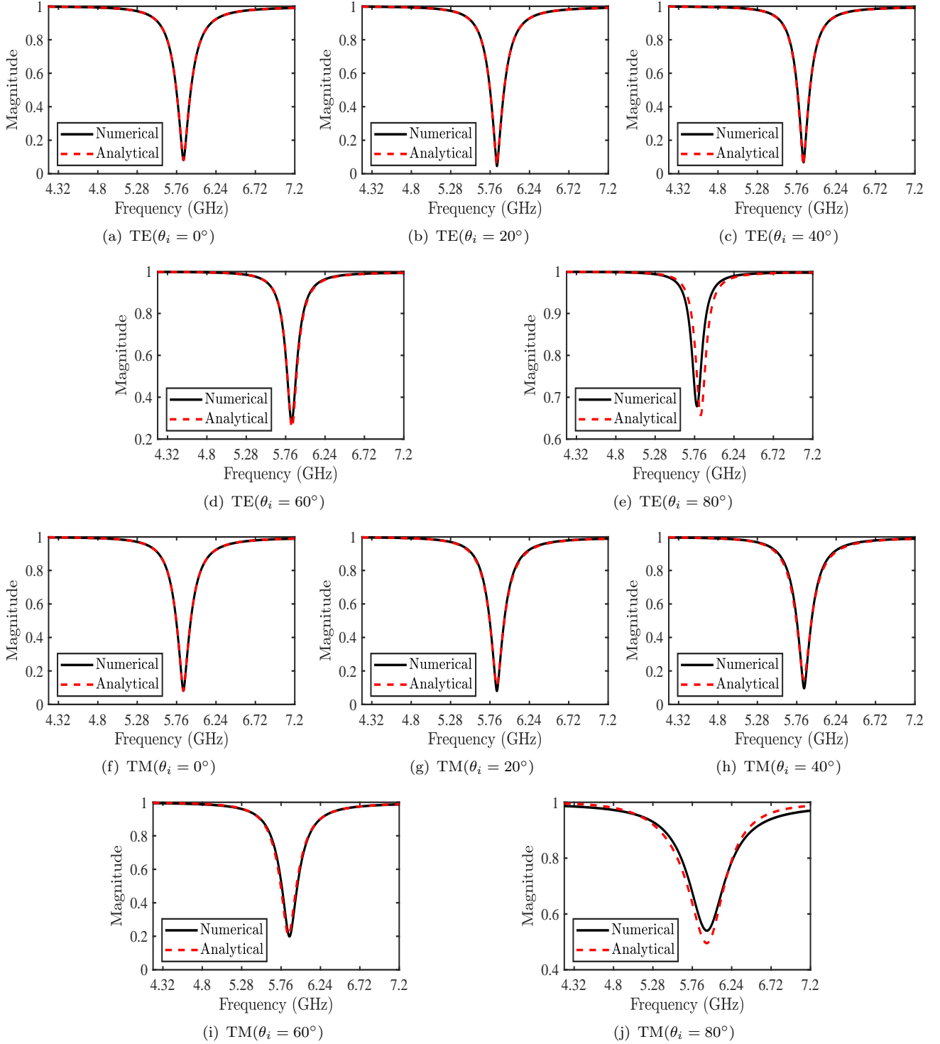
Figure 5. Comparison between numerically simulated and analytically calculated reflection coefficients for different values of the incidence angle \theta_i : (a),(b),(c),(d) and (e) Case of TE. (f),(g),(h),(i) and (j) Case of TM.
