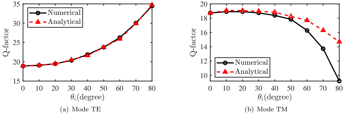
Figure 7. Corresponding change of the quality factor of the unit-cell as a function of the incidence angle \theta_i : 7(a) Case of TE–polarized wave excitation and 7(b) TM–polarized wave excitation.
