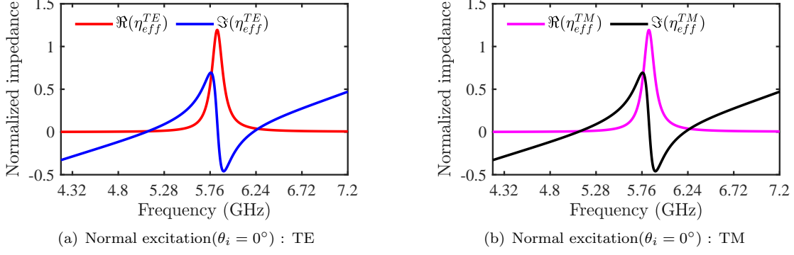
Figure 4. Normalized equivalent effective impedance of the unit-cell as a function of frequency : 4(a) Case of TE mode excitation, and 4(b) case of TM mode excitation.
