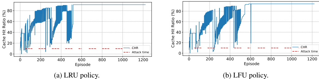
Figure 21: Performance of CHR using different caching policies.
