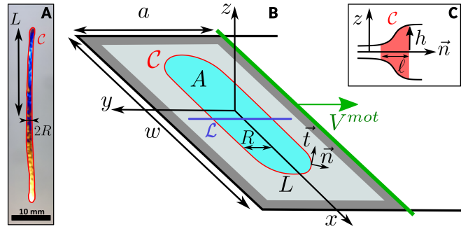
FIG. 1. Experimental setup and notations used in the text. (A) Image of the film recorded by the top camera. (B) Schematic view of the setup. The black and green thick lines represent respectively the static and mobile edges of the frame. The thin film (colored domain in (A), light blue in (B)) is separated from the light gray thick film by the red contour C . (C) Schematic thickness profile along L , in the vicinity of C , on the right-hand side of Fig. 1B.
