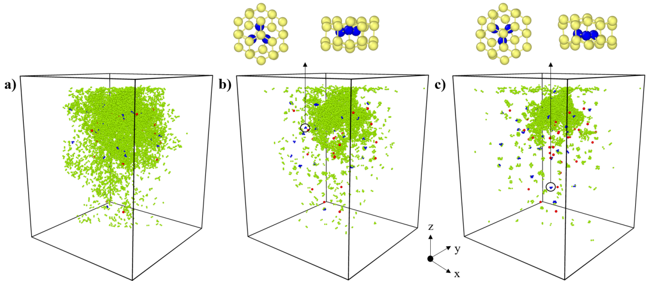
FIG. 8. Snapshots of the defects in the 5 keV irradiation system with a fluence of 50 \times 10^{12} \text{ ions cm}^{-2} a) before annealing, b) after 0.5 ns annealing and c) 3 ns annealing at 1400 K. The Ga atoms are represented with red, the interstitials with green and the tri-interstitial clusters with blue. In the black circles and above the simulation box are some of the symmetric tri-interstitials identified by the developed method observed following the \langle 111 \rangle (left image) and \langle 11 - 2 \rangle (right image) directions.
