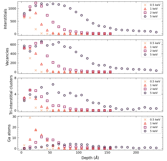
FIG. 4. Interstitials, vacancies, tri-interstitial clusters and irradiated Ga atoms average depth distributions (ten simulations), for different irradiation energies with a fluence of 50 \times 10^{12} \text{ ions cm}^{-2} .
