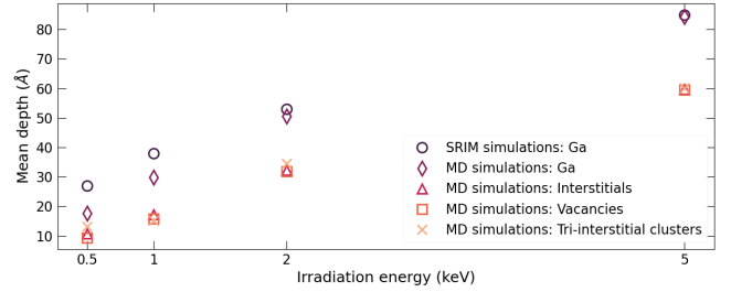
FIG. 3. Ga mean stopping depth and defects mean formation depth as a function of irradiation energy for MD and SRIM simulations.
