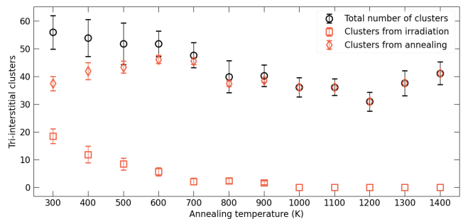
FIG. 6. The number of tri-interstitial clusters after 0.5 ns of annealing at different temperatures for the 5 keV irradiation energy and a fluence of 50 \times 10^{12} \text{ ions cm}^{-2} . The black circles represent the total number of tri-interstitial clusters, the orange squares the clusters produced from irradiation and the orange diamonds the number of clusters produced during annealing.
