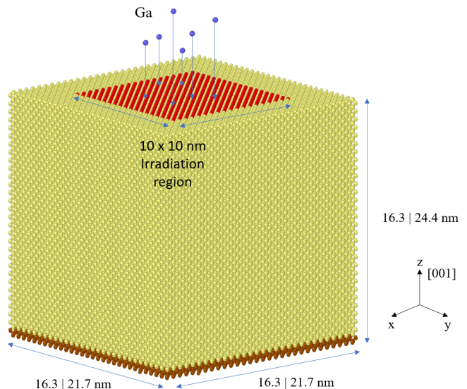
FIG. 1. MD model of irradiation. Blue atoms correspond to the irradiated Ga atoms, brown atoms to the bottom fixed layer, yellow atoms to the Newtonian region and the red atoms to the surface atoms where the irradiation occurs. The different lengths at the sides indicate the side lengths of the different models employed in this study.
