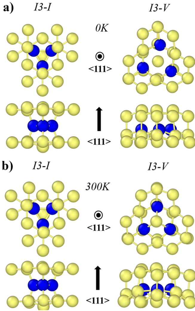
FIG. 2. a) W center defect structure candidates, produced by minimization of a distorted tri-interstitial cluster placed in between the \{111\} planes using the Tersoff potential. W center with the I3-I (left) and I3-V (right) structure at 0K. b) The same defects at 300K where the average configurations (from 10 different structure snapshots at 300K) of the clusters are shown. The blue balls correspond to the tri-interstitial defect atoms.
