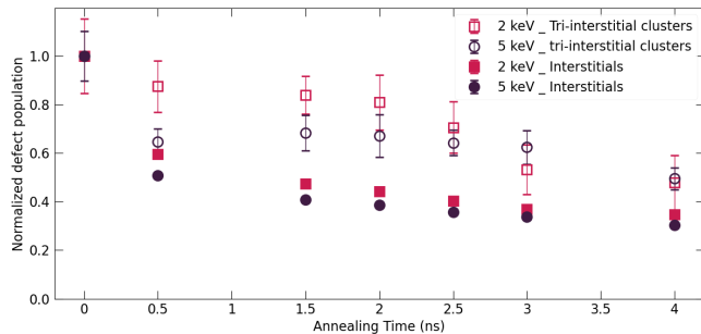
FIG. 7. Normalized number of tri-interstitial clusters and the overall interstitials after different annealing times at 1400 K for different irradiation energies and a fluence of 50 \times 10^{12} \text{ ions cm}^{-2} .
