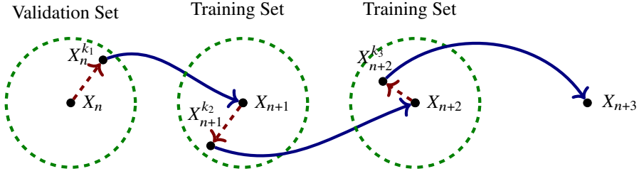
Figure 3. The schematics of the flow of analogs. When applying the algorithm for estimation of committor (equation (3)) the first step consists of starting from the state in the Validation Set (VS), finding the analog in the Training Set (TS) and applying the time evolution operator. All subsequent transition occur within the TS..
