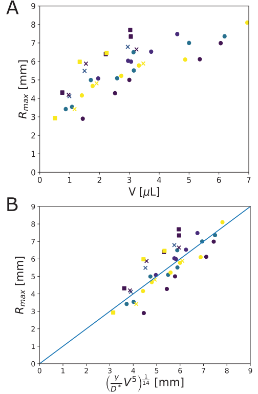
Fig. 4: Maximal drop radius. (A) Values of R_{max} obtained from our experiments on different substrate materials (x : PVS E = 0.2 Mpa, o : PVS E = 0.9 Mpa, \square : PDMS E = 1 Mpa) and oil viscosities ( \eta = 2.3 , yellow; 5.4: blue; and 10.5 mPa · s: purple). R_{max} seems independent on the oil viscosity. (B) Rescaled values according to eq. (6). The blue line is a guide for the eye.
