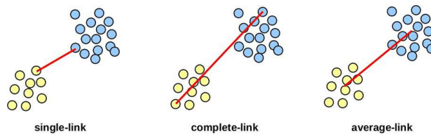
Figure 4: Examples of single, complete and average linkage methods. from [25].
