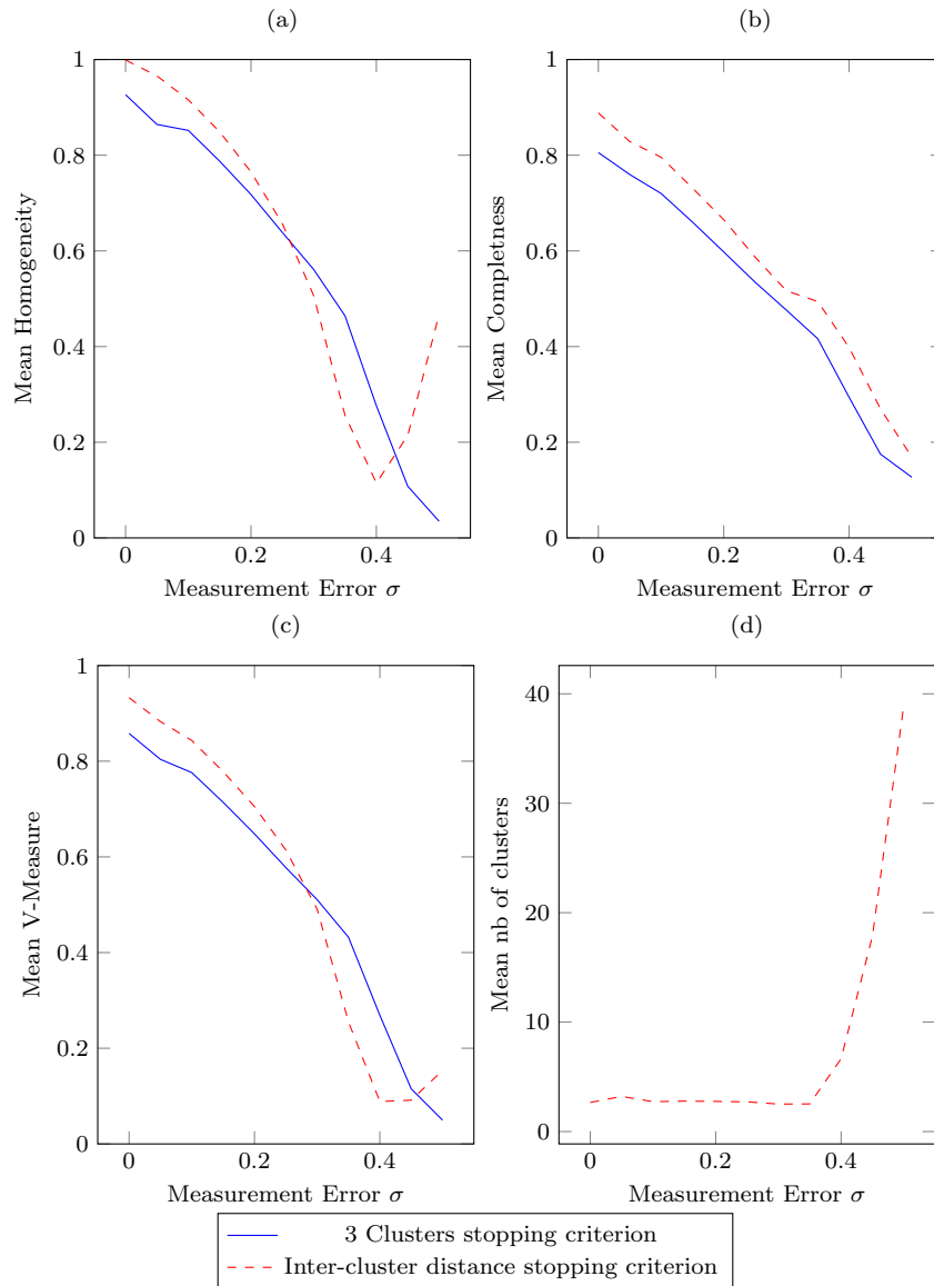
Figure 8: Performance evaluation of our clustering solution (mean interpolation difference + weighted mean linkage method for AHC) under various levels of measurement noise, with a stopping criterion based on maximum number of sensors (solid blue line) and one based on threshold inter-cluster distance (dashed red line).
