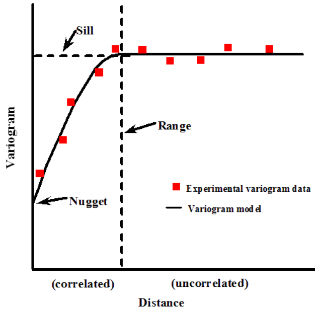
Figure 2: Illustration of the variogram model based on experimental variogram points. The variogram consists of three parameters: nugget, sill, and range. The closer (temporally) the distance between two observations, the more correlated the values. Beyond a certain threshold, defined by the range, observations that are too distant are no longer correlated.
