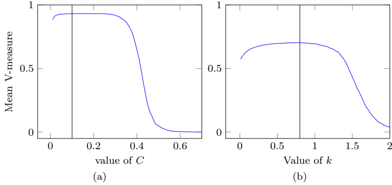
Figure 7: (a) Average V-measure performances with zero noise, while varying the threshold distance parameter C .
