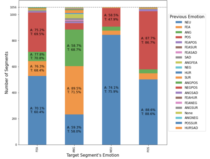
Figure 5: Prediction accuracy of the target emotions based on the previous segment's emotion, A: prediction on acoustic, T: prediction on speech transcripts, % in UA
