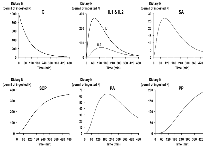
FIGURE 12. Predictions of the evolution kinetics for sampled compartments calculated using either the optimum set of parameters (black curve) or the estimated set of parameters (grey curve) when "noise-free" data ( d_0 ) are injected into the objective function.
