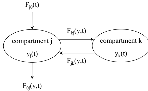
FIGURE 1. Example of diagram of the j^{\text{th}} and k^{\text{th}} compartments of an n -compartment model (using the notations described in section 1.1.2).
