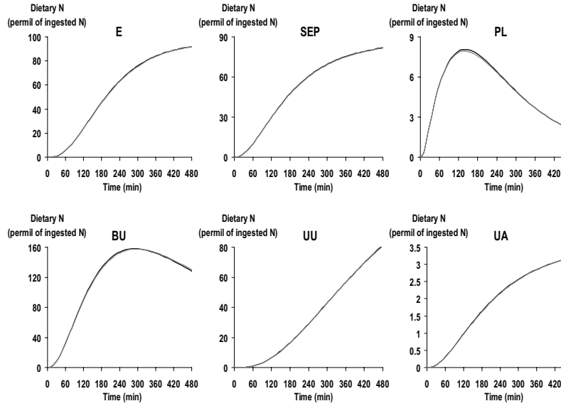
FIGURE 17. Predictions of the evolution kinetics for sampled compartments calculated using either the optimum set of parameters (black curve) or the estimated set of parameters (grey curve) when "high-noise" data ( d_2 ) are injected into the objective function.
