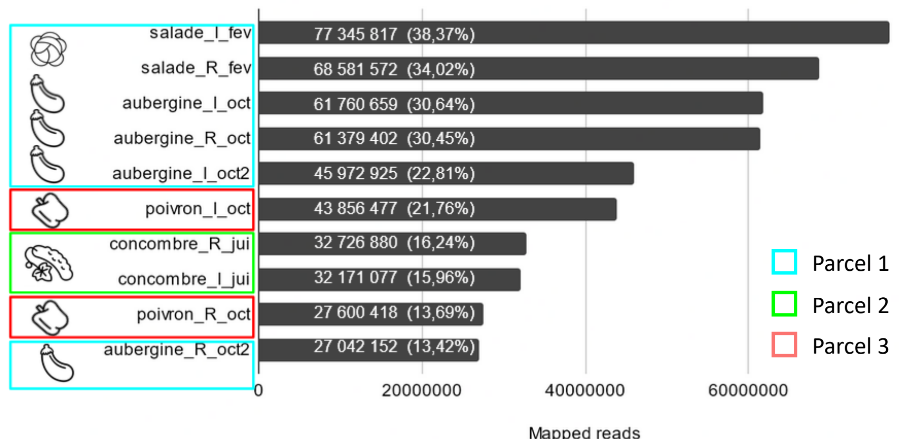
Fig. 3 : Comparative Analysis of Short-Read from salade soil samples mapping across 10 Long-Read Datasets Using BWA-mem2, with alignment filtering criteria of ≥90% identity and alignment length >130 bp.
