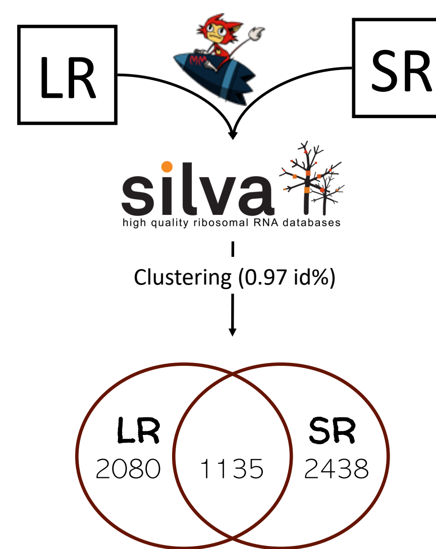
Fig. 4 : Workflow for virtual metabarcoding analysis, from the identification of ribosomal DNA in both SR and LR datasets using MMseq2 toolkit [6] and SILVA database as reference to the OTUs comparison through a Venn diagram. Subsequently, barcodes are clustered at a 97% identity threshold using the cd-hit software [7]. Finally, OTU comparison is performed through a Venn diagram.
