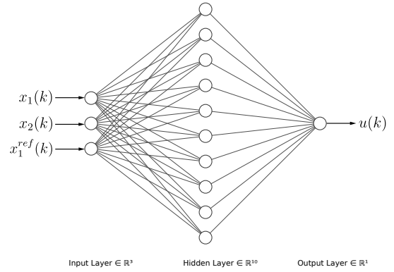
Fig. 1. Architecture of the NN used to simulate the MPC controller of Example 1.
