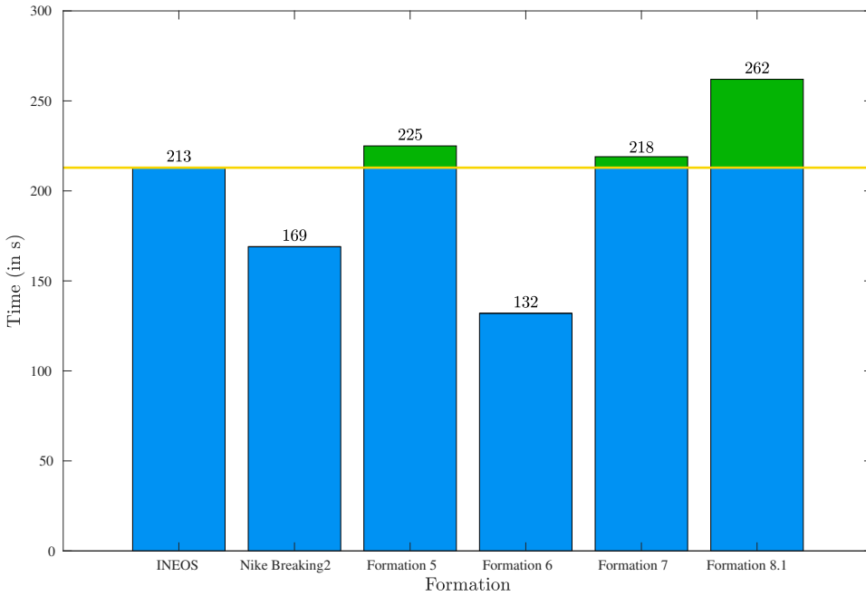
Figure 16. Time savings for different formations with respect to a solo runner computed with the models of [25] and [26]
