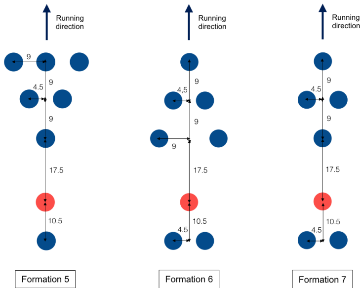
Figure 14. Top view of pacer formations in scaled wind tunnel testing (distances in cm). The designated runner is indicated by the red circle and the pacers are indicated by the blue circles. Novel complex pacer formations
