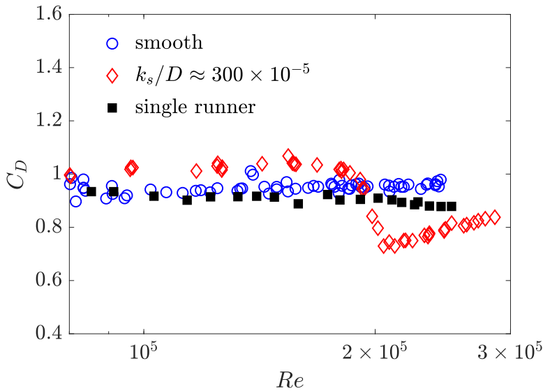
Figure 4. Measured drag coefficient C_D as a function of Re for a finite-length circular cylinder with an aspect ratio L/D \simeq 2.9 : smooth cylinder \circ , rough cylinder \diamond ; and for the solo runner manikin \blacksquare
