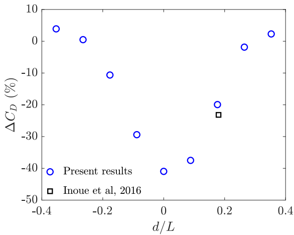
Figure 11. Relative variation of C_D with respect to a solo runner as a function of the normalized lateral position d/L of the leading runner (see Fig. 8, case 3)
