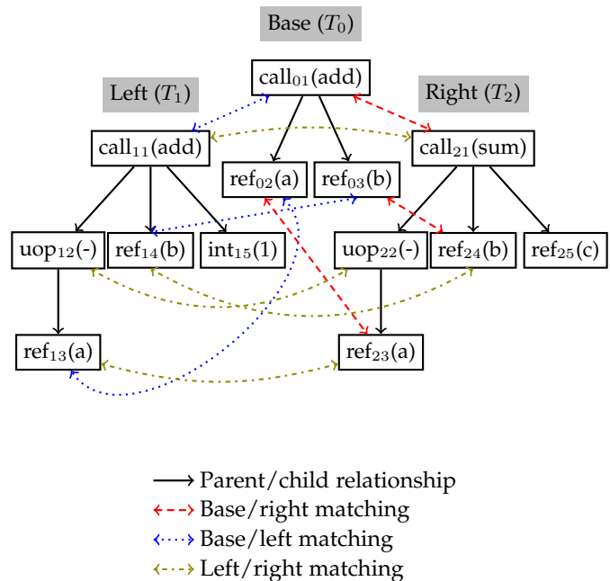
Fig. 1: Pairwise matchings between simplified ASTs of the function calls in Table 1. Each node is subscripted with a unique identifier xy , where x indicates the tree the node belongs to and y is unique within tree x .
