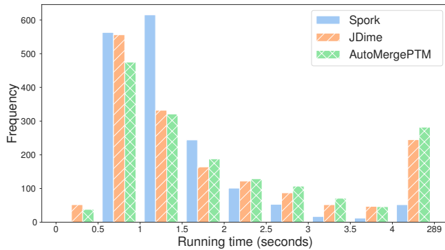
Fig. 15: Histogram of file merge running times for SPORK, JDIME and AUTOMERGEPTM. Lower is better. Each histogram bin contains the frequency of values in the range [L, R) , where L and R are the values to the left and right of the bin, respectively.
