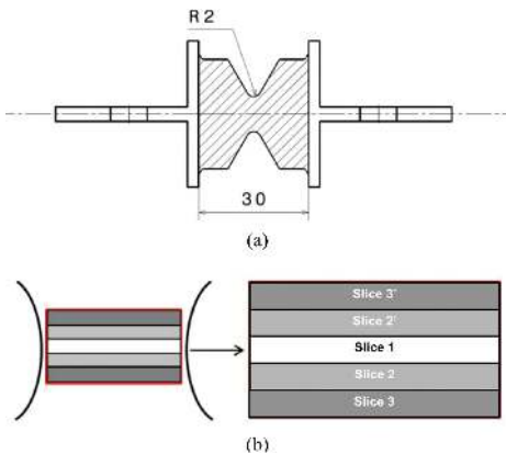
Figure 1. (a) Geometry of the AE2 sample, (b) observed zone and definition of the different slices.
