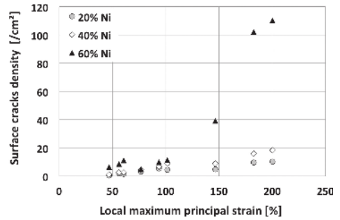
Figure 4. Density of surface cracks with respect to the maximum principal local strain for the three percentages of fatigue life (% Ni).
