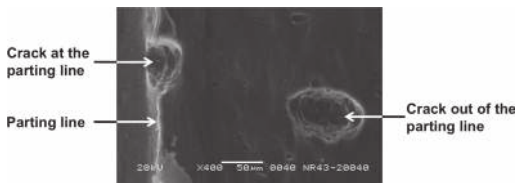
Figure 3. SEM picture of the typical locations of crack initiation sites: at the parting line or out of the parting line.
