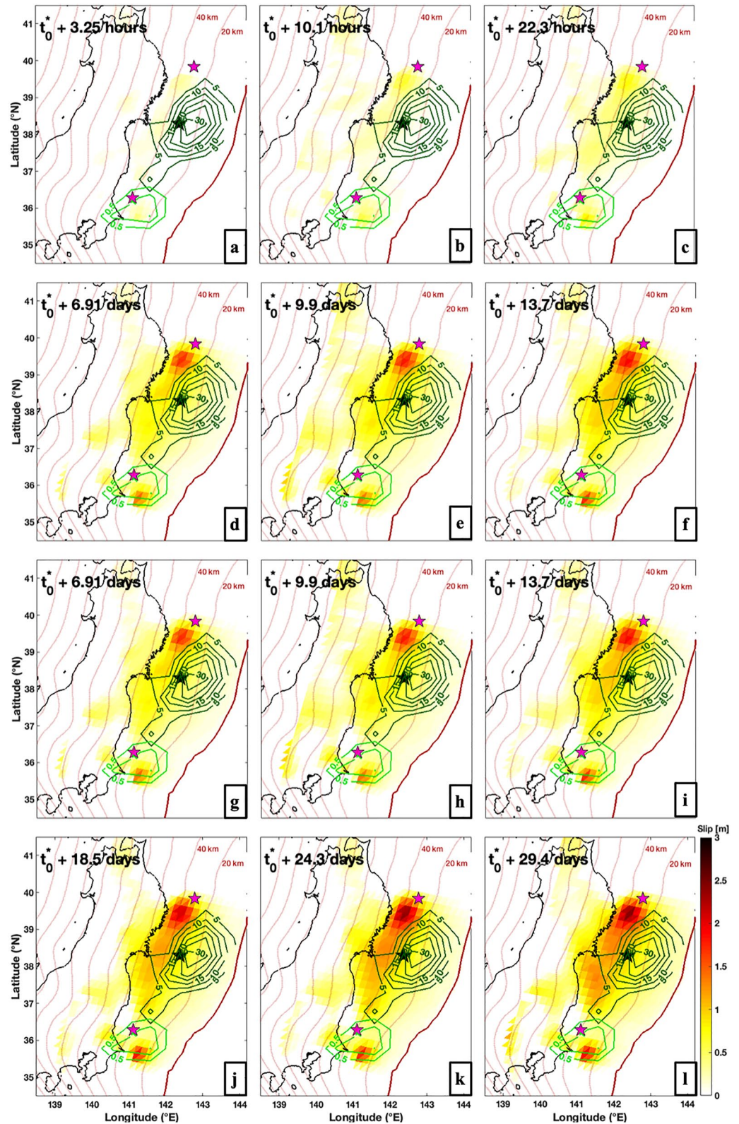
Figure 9. Spatio-temporal evolution of afterslip during the first month on 12-time windows: Aftershock(s) coseismic offsets are removed from the postseismic deformation. Green lines represent slip contours of the Tohoku-Oki mainshock and Ibaraki-Oki aftershock in meters. Stars correspond to the three main events. Color scale indicates the slip amplitude in meters.
