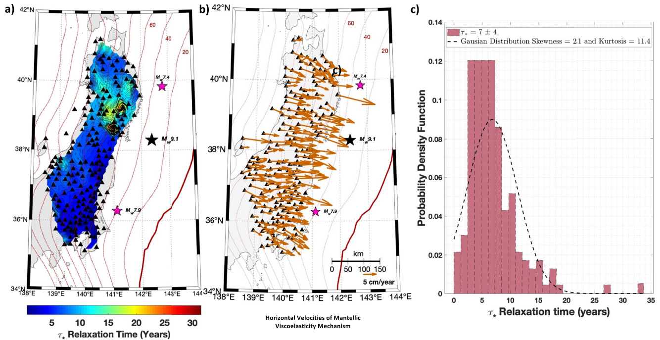
Figure 7. Parameters and Statistics obtained on 192 stations successfully inverted for Time Series up to \sim 2020 . (a) Relaxation time \tau_* interpolated map. (b) Map of horizontal velocities v_1 associated with a mantelic viscoelastic mechanism. (c) Relaxation time \tau_* statistics and distribution.
