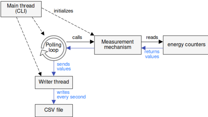
Figure 4. Architecture of our measurement tool
