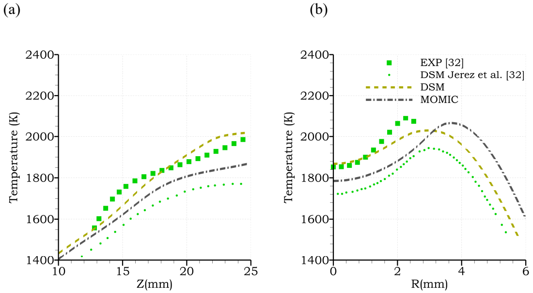
Fig. 4 Temperature profiles (a) along the flame centerline Z and (b) over a radial direction R at the position Z/H=0.6 . Square symbols correspond to the experimental data [32], whereas dash-dot, dash, and dot lines correspond to numerical results.
