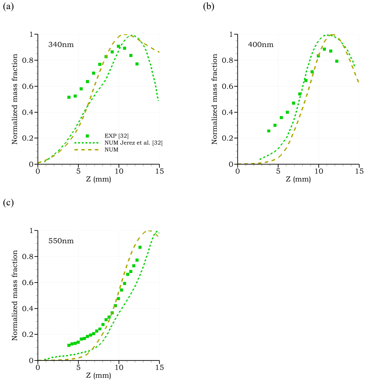
Fig. 7 Normalized mass fraction axial profiles for wavelengths (a) 340 nm (b) 400 nm and (c) 550 nm. Square symbols correspond to the experimental data [32], whereas dash, and dot lines correspond to numerical results.
