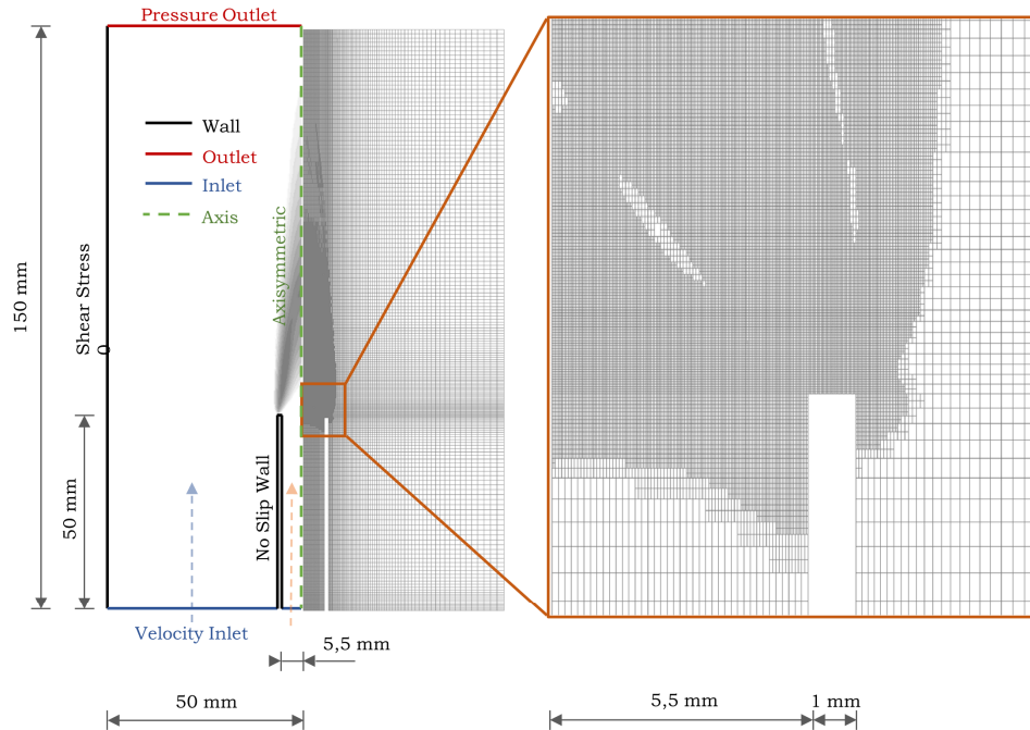
Fig. 1 2-D axisymmetric computational domain, boundary conditions, and refined computational mesh.
