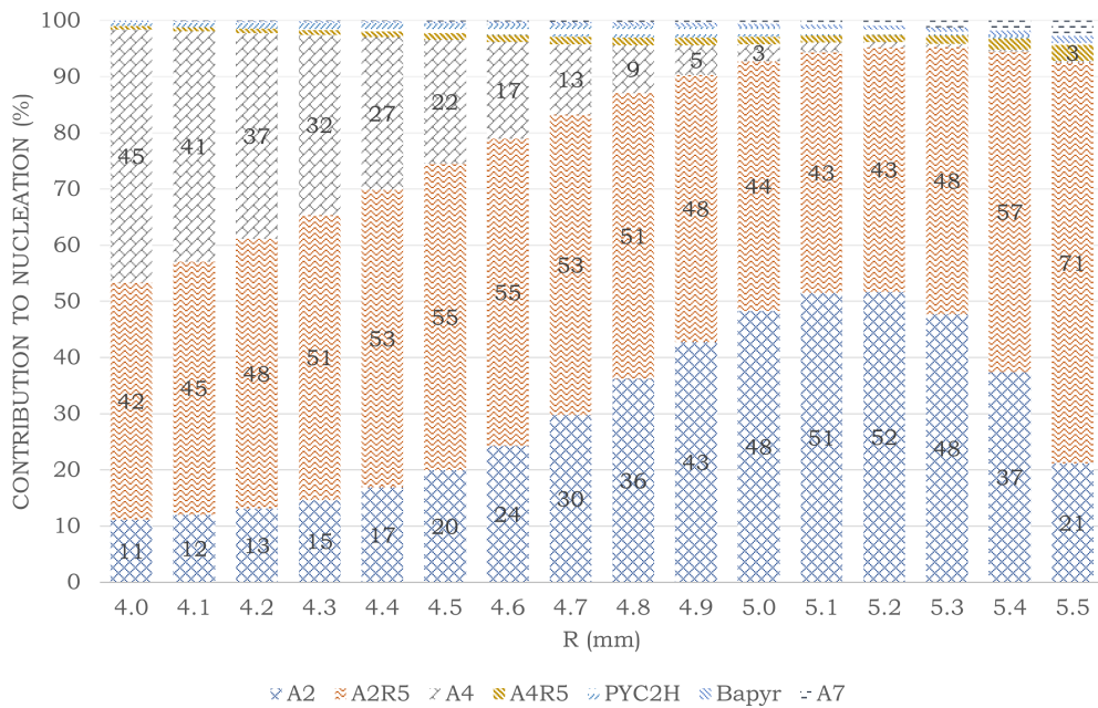
Fig. 10 PAH normalized contribution to soot nucleation rate over a radial direction at the position Z = 2 mm.
