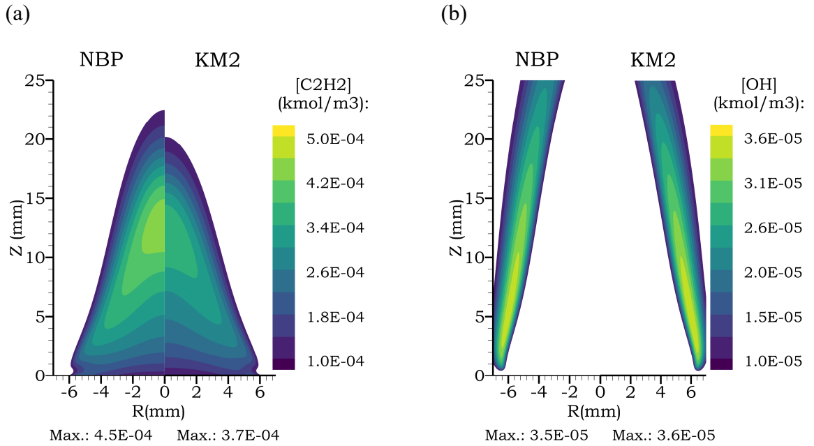
Fig. 3 Molar concentrations (kmol/m 3 ) obtained using the NBP and KM2 chemical kinetic mechanisms. (a) C_2H_2 and (b) OH.
