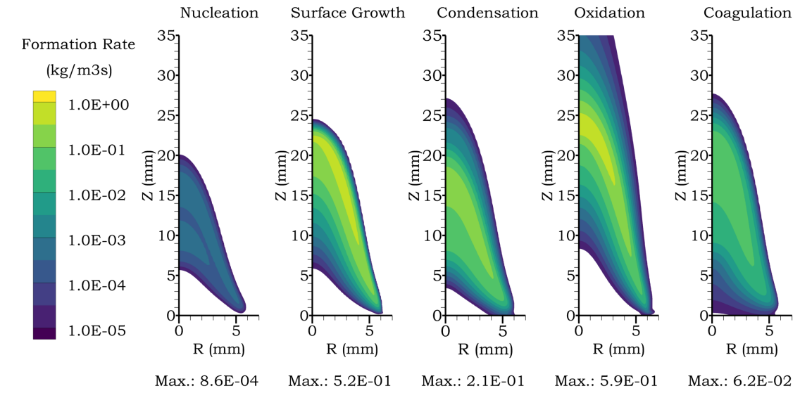
Fig. 6 Distribution of soot formation rates ( \text{kg}/\text{m}^3\text{s} ) obtained using the DSM soot formation model and KM2 gas phase kinetic mechanism.
