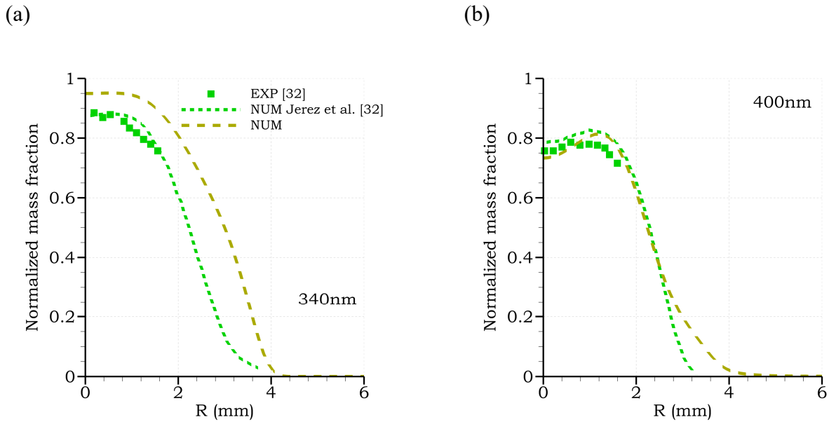
Fig. 8 Normalized mass fraction radial profiles at Z/H = 0.3 for wavelengths (a) 340 nm and (b) 400 nm. Square symbols correspond to the experimental data [32], whereas dash, and dot lines correspond to numerical results.
