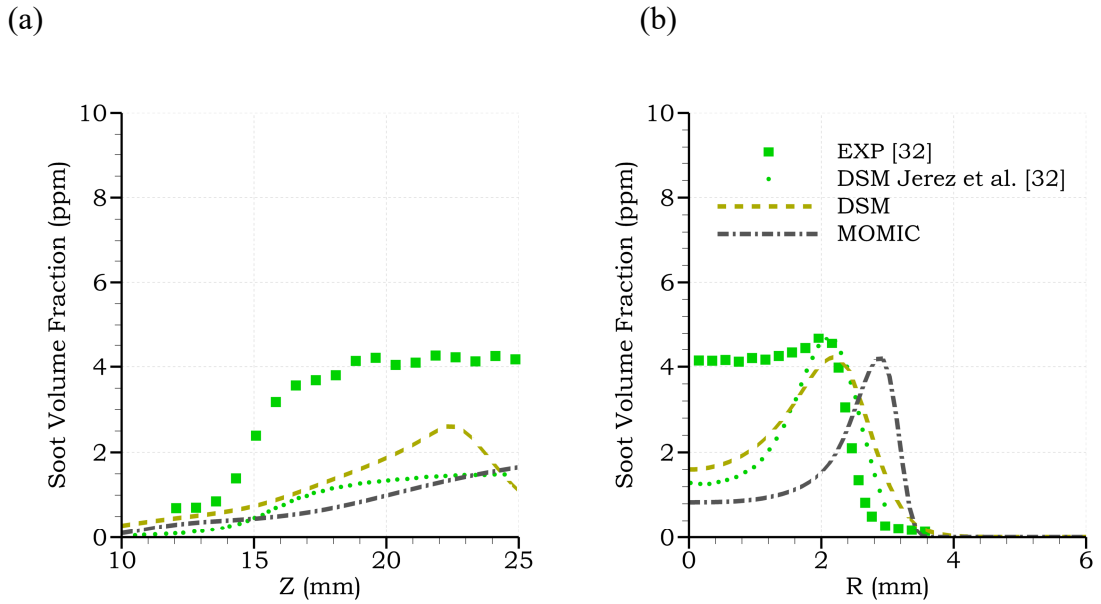
Fig. 5 Soot volume fraction profiles (a) along the flame centerline Z and (b) over a radial direction R at Z/H=0.6 . Square symbols correspond to the experimental data [32], whereas dash-dot, dash, and dot lines correspond to numerical results.
