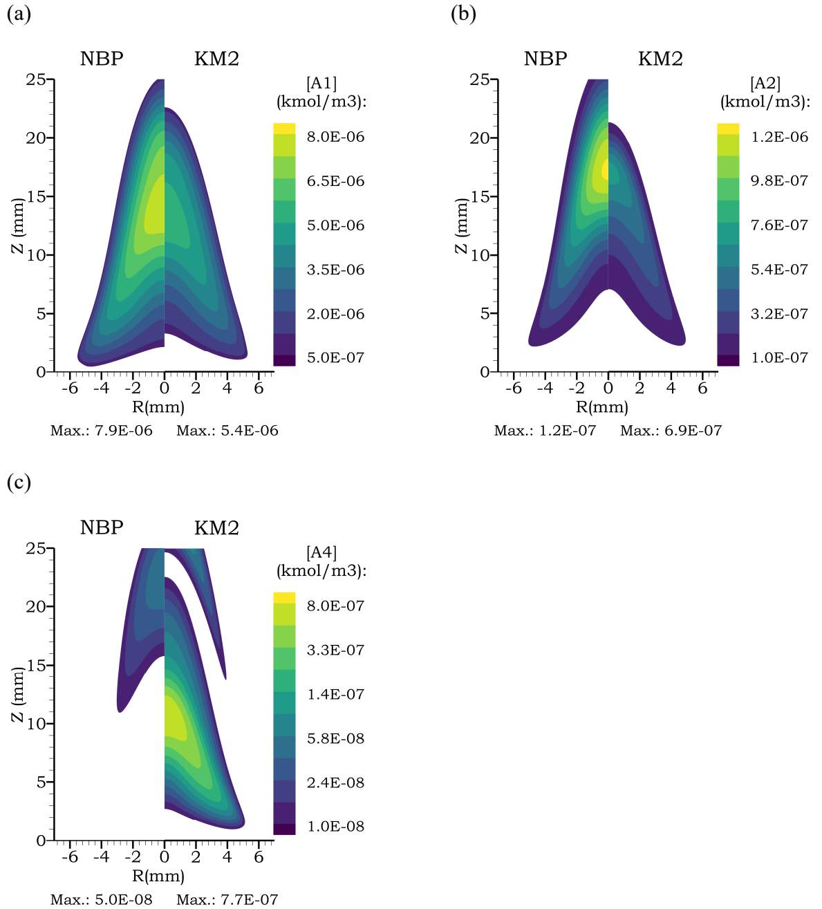
Fig. 2 Molar concentrations (kmol/m 3 ) obtained using the NBP and KM2 chemical kinetic mechanisms. (a) Benzene (A1), (b) naphthalene (A2), and (c) pyrene (A4).
