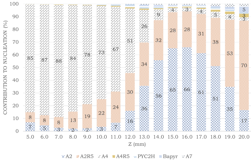
Fig. 9 PAH normalized contribution to soot nucleation rate over the flame centerline.
