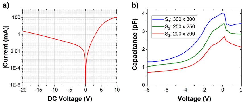
Figure 4: Electrical characterization of the PIN-based SiGe EOM. (a) I-V characterization in the 5.9 mm long device. (b) Evolution of the capacitance in test structures (squared MESA) with different dimensions, as a function of the applied voltages (length of 200 \mu\text{m} , 250 \mu\text{m} and 300 \mu\text{m} ).
