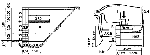
Fig.14 Geometry
