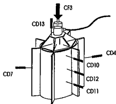
Fig-8 Compression test
