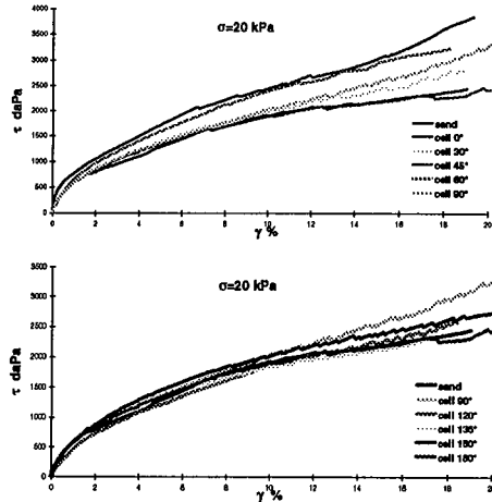
Fig. 5 Results of shearing tests
