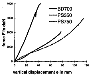
Fig.9 Results of compression tests
