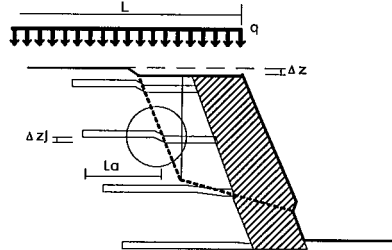
Fig.12 Two blocks method
