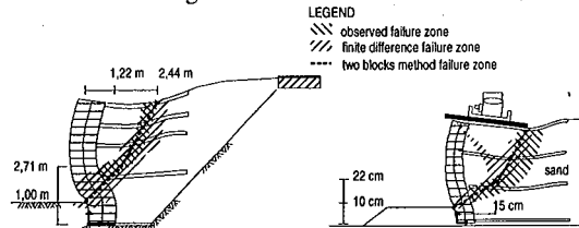
Fig.16 Comparison of the different line of failure
