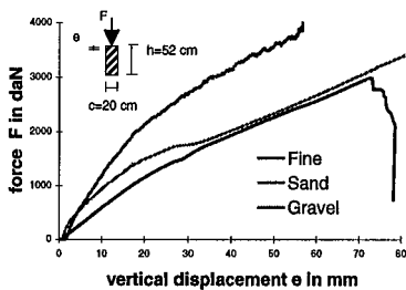
Fig-8 Compression test
