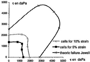
Fig.7 Comparison of experiments and theory
