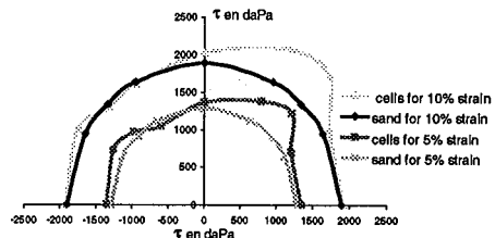
Fig-6 Polar diagram
