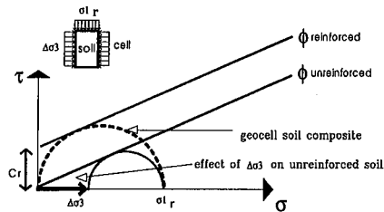
Fig.10 Definition of parameters
