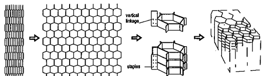
Fig.1 Reinforced geocells soil structures
