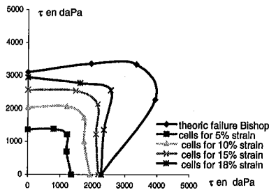
Fig.11 Comparison of experiments and theory
