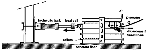
Fig. 3 Plan of the simple shear box
