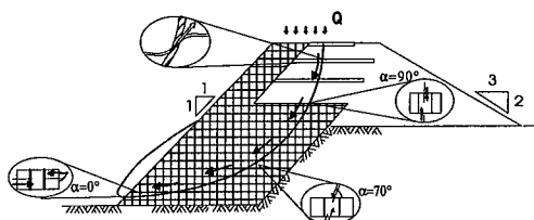
Fig.2 Failure mode
