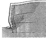
Fig.15 Failure zone predicted by finite difference
