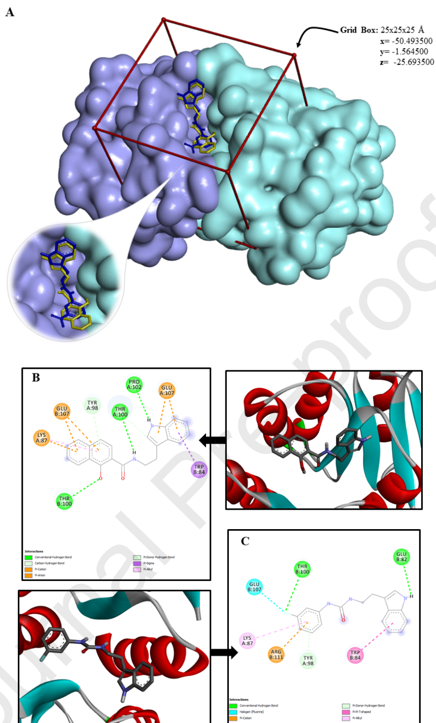
Figure 4. A) Binding pocket of the homo-dimer PhoP of E. coli (PDB: 2PKX), and superimposed bond ligands: A (blue color) and 3b (yellow color). B) and C) present the docked binding mode of compound A and 3b respectively.
