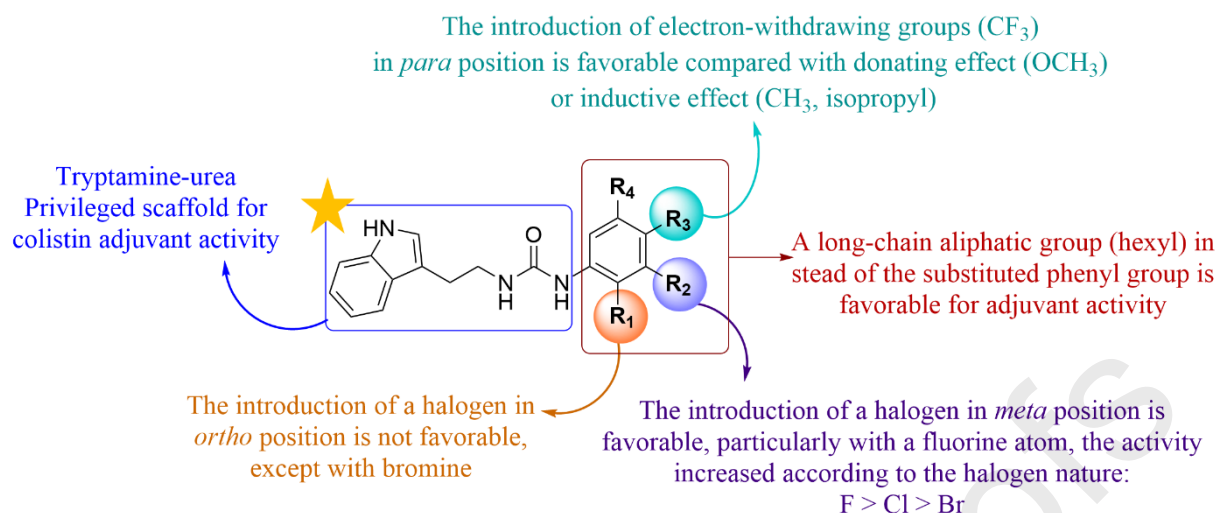
Figure 2. SARs of tryptamine-urea derivatives against chromosomally-mediated colistin resistance K.pneumoniae strain (KP BA03057).
