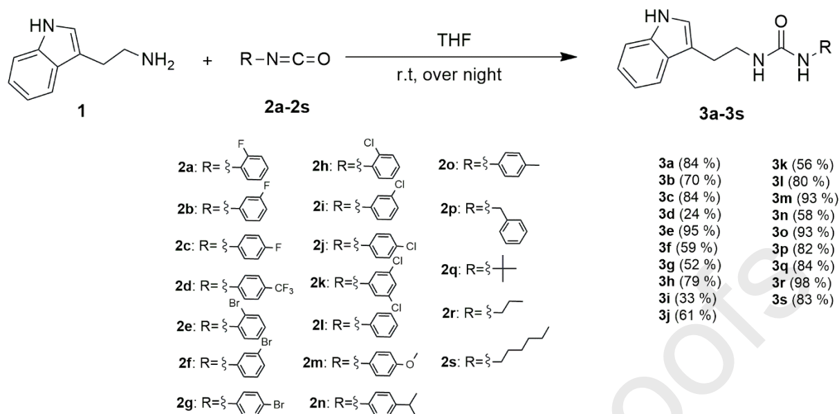
Scheme 1 Synthetic route of compounds 3a-3s
