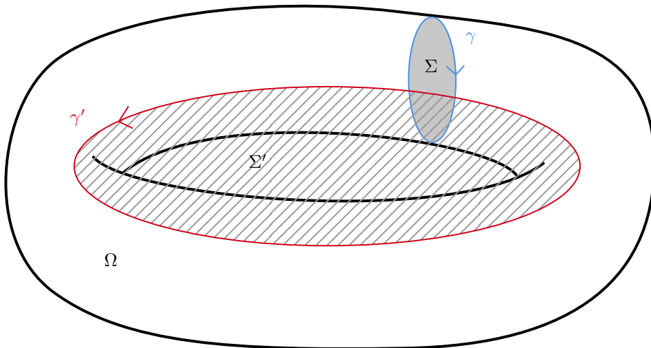
Figure 1: Illustration of the curves \gamma and \gamma' , and the surfaces \Sigma and \Sigma'
