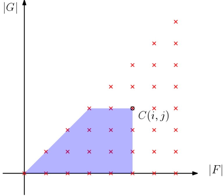
FIGURE 2. An illustration of the recurrence argument. The constant C(i, j) can be bounded by a linear combination of the C(i', j') with j' \leq j , i' \leq i , and i' + j' < i + j .
