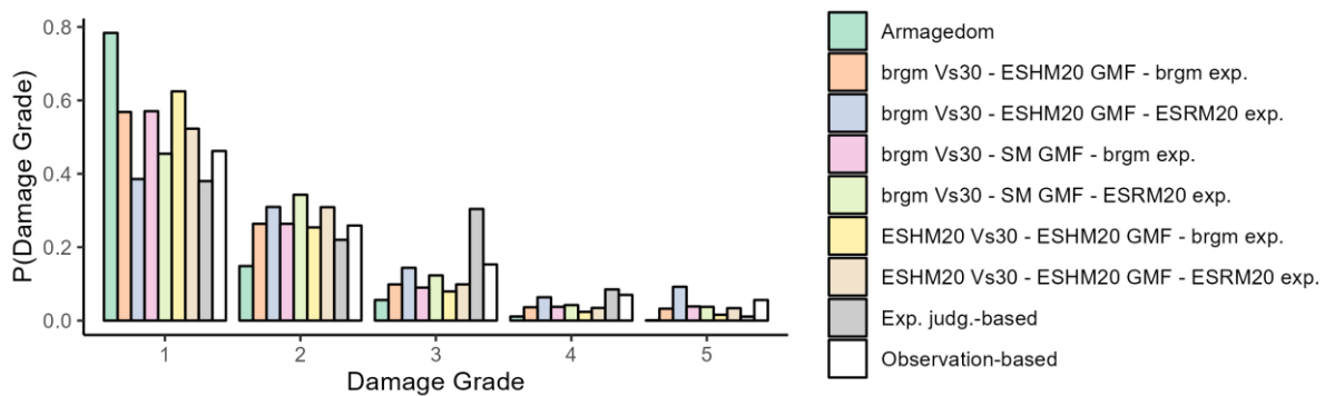
Figure 5. Probabilities and number of buildings with EMS-98 damage grades for the configurations of the simulations with aggregated exposure including the total number of buildings in Le Teil
