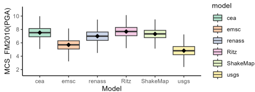
Figure 2. Boxplots for a) the Mercalli-Cancani-Sieberg (MCS) macroseismic intensity as a function of the PGA given by the ground motion-to-intensity conversion equation by Faenza and Michelini [2010] (“FM2010”) (the edges of the box are located at the first and third quartile, respectively, the line at the middle of the box is located at the median, the point marker is located at the mean of the sample, the whiskers extend up to 1.5 times the distance between the first and third quartile approximating the 95 % confidence interval).
