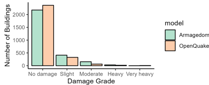
Figure 3. Estimated number of buildings in each damage grade based on two scenario analyses using the Armagedom risk analysis tool on the VISIRISKS platform (Armagedom) and a model with equivalent exposure and fragility models (selected from the ESRM20) combined with elements of the ESHM20
