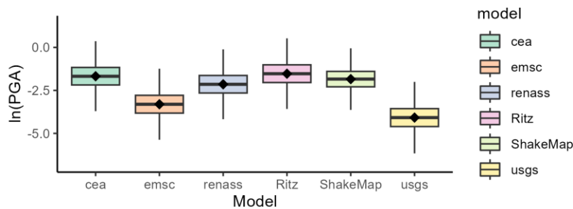
Figure 1. Boxplots for the generated samples for the considered ground motion intensity measures at all exposure centroids based on the scenario simulations (the edges of the box are located at the first and third quartile, respectively, the line at the middle of the box is located at the median, the point marker is located at the mean of the sample, the whiskers extend up to 1.5 times the distance between the first and third quartile approximating the 95 % confidence interval).
