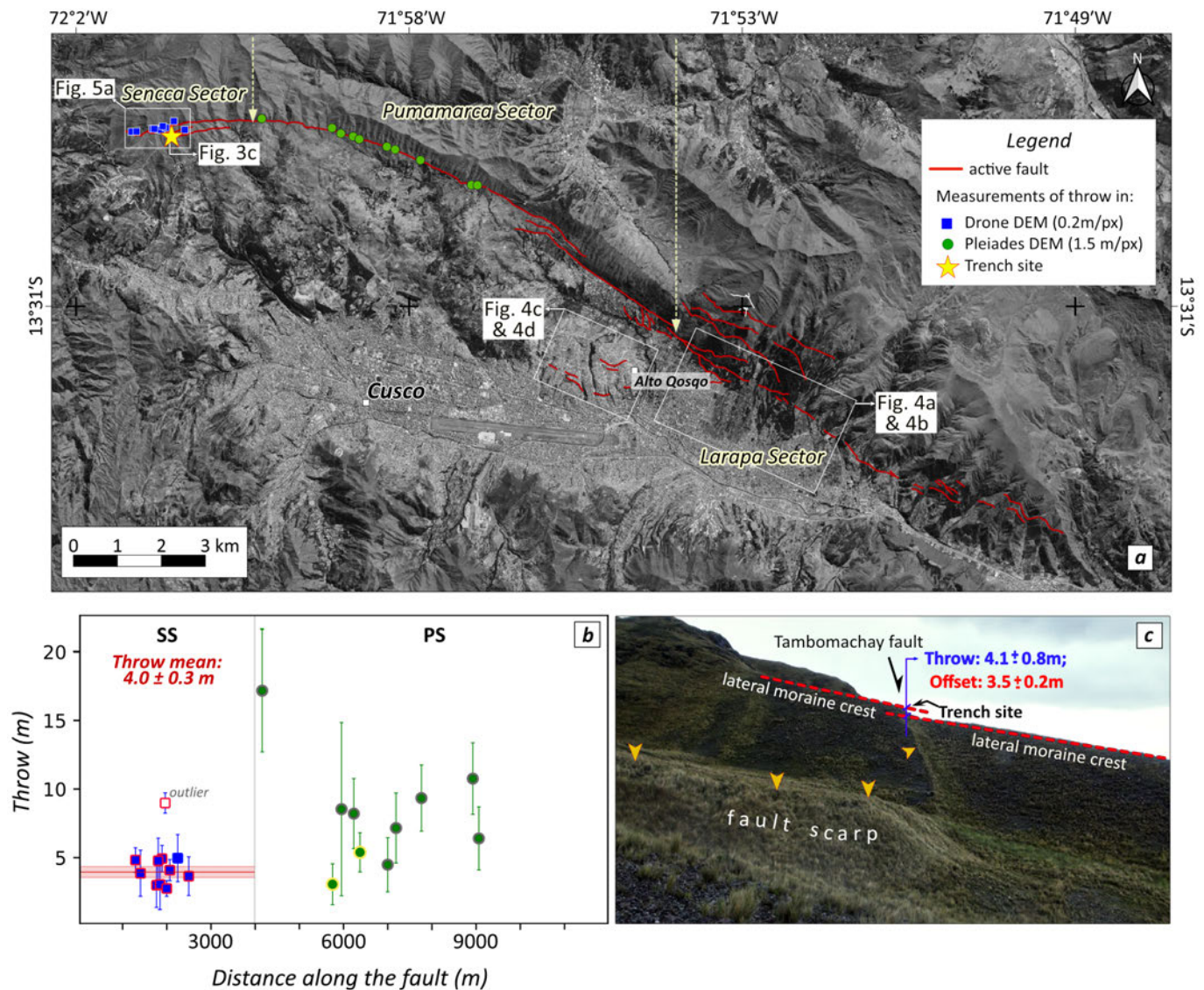
Figure 3 – a ) Optical satellite imagery (from Google, DigitalGlobe) of the detailed mapping of Tambomachay Fault scarps along the sectors: Sencca (SS), Pumamarca (PS) and Larapa. The yellow dashed lines delimit the sectors along the fault trace. The blue squares indicate the location of scarp offset measurements from the 11 fault-perpendicular profiles extracted from the high-resolution DEM (0.2 m/px). The green circles indicate the location of scarp offset measurements from the 10 fault-perpendicular profiles extracted from the high-resolution DEM (1.5 m/px). The yellow star indicates the location of the paleoseismic trench. b ) Scatter plot of the variability of throw measurements with their respective uncertainties along the Tambomachay Fault. The blue squares with red borders represent measurements on Holocene fluvio-glacial deposits, while the borderless blue square represents a measurement on bedrock. The red line represents the mean throw value in the Sencca Sector and its buffer represents the error of the weighted-mean. The green circles with yellow borders represent measurements on Quaternary alluvial deposits, while green circles with grey borders represent measurements on bedrock. c ) Field photograph with profile view of a lateral moraine in the Sencca Sector. The yellow triangles indicate the Tambomachay Fault scarp. The throw measurement value, and location of the paleoseismic trench on the displaced lateral moraine crest are also indicated.
