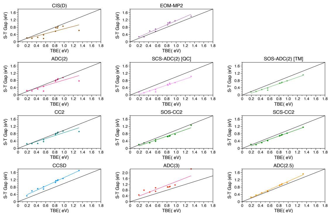
FIG. 4. Correlation graphs between the STGs and the TBEs (both in eV) for various computational methods determined on the full set of molecules.
