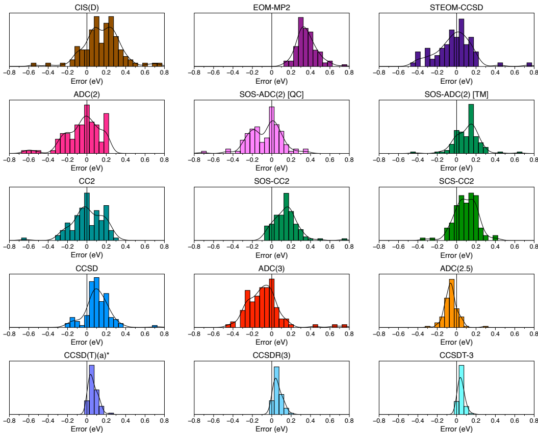
FIG. 3. Distribution of the error (in eV) in VTEs (with respect to the TBEs) for various computational methods determined on the full set of molecules and states.
