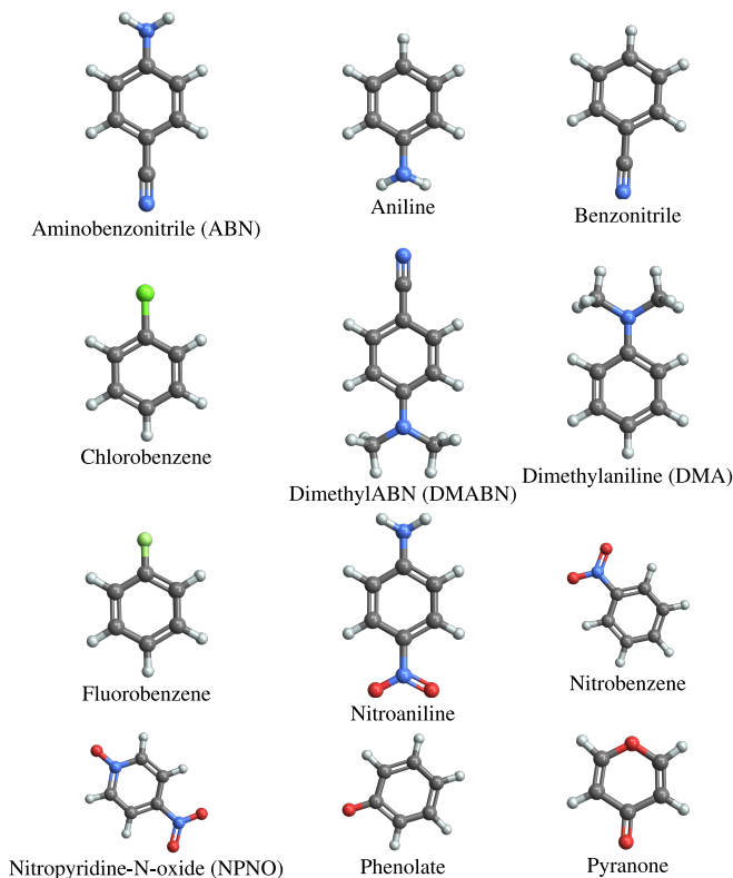
FIG. 1. Representation of the systems investigated in the present study.
