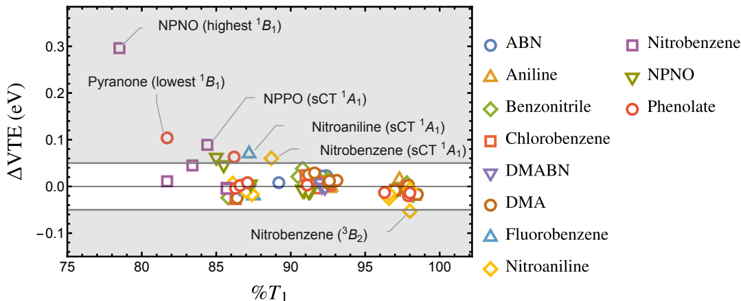
FIG. 2. Difference between the CCSDT and CC3 VTEs, \Delta VTE (in eV), as a function of the percentage of single excitation involved in the transition ( \%T_1 ) computed at the CC3/aug-cc-pVDZ level. The largest available basis set is considered to determine the difference in VTEs. The grey areas indicate errors larger than 0.05 eV. Selected outliers are specifically labeled.
