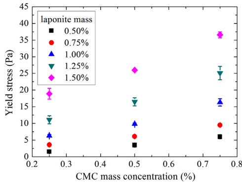
Fig. 4. Yield stresses as a function of CMC mass concentration for D+20.
