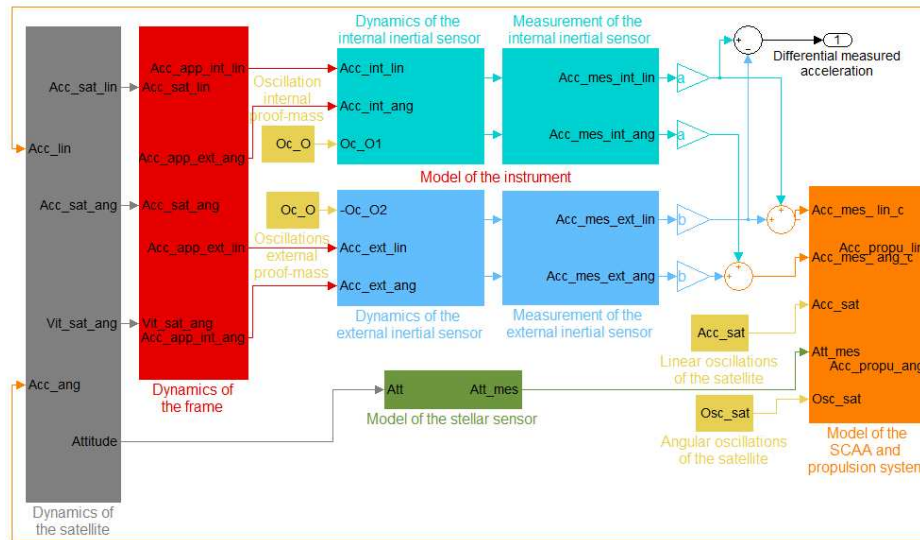
Fig. 1. Scheme of the calibration simulator
