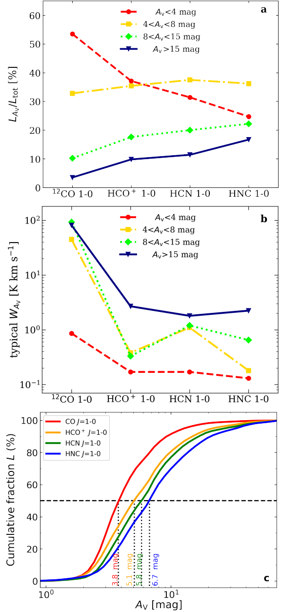
Fig. 5. Line emission properties as a function of A_V . (a) Fractions (in %) of line luminosities emitted in each A_V mask. (b) Typical (the mode) line intensity in each A_V mask. (c) Cumulative line luminosity.
