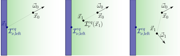
Figure 13: Different examples of contribution to the radiative intensity calculated at a location \vec{x}_0 and direction \vec{\omega}_0 ; (left) - Reinforcement due to radiation emitted at the boundary I_{v,\text{left}}^{\text{eq}} and attenuated along the path; (center) - Reinforcement due to radiation emitted within the volume I_v^{\text{eq}}(\vec{x}_1) and attenuated along the path; (right) Reinforcement due to a contribution scattered from a direction \vec{\omega}_1 at a location \vec{x}_1 .
