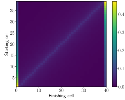
(d) Cases 7 and 8 , where \mathcal{N} = 1 and walls are black.
