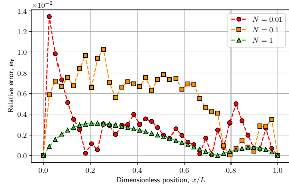
(b) Corresponding error profiles for different values of \mathcal{N} in the case of T_{\text{right}} = 2 \times T_{\text{left}} .
