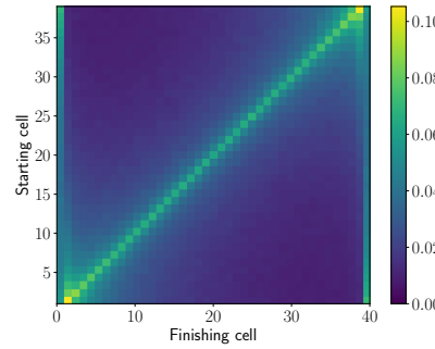
(f) Case 10 where \mathcal{N} = 0.01 and walls are gray with \epsilon_{\text{left}} = \epsilon_{\text{right}} = 0.1 .
