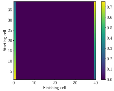
(h) Cases 11 and 12 , where \mathcal{N}' = 10 , walls are black and k_s = 1 .
