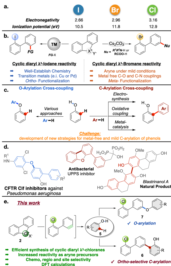
Figure 1: a) Electronic properties of iodine, bromine and chlorine; b) Reactivity of cyclic diaryl \lambda^3 -iodonium and bromonium salts; c) Common C-O and C-C couplings of phenols; d) Selected examples of biologically active terphenyls; e) This work
