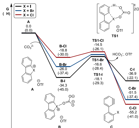
Figure 3: Calculated energy diagram (in kcal mol -1 ) for the formation of arynes C from hypervalent halonium 2a (red color), 3a (black) and 4a (blue).
