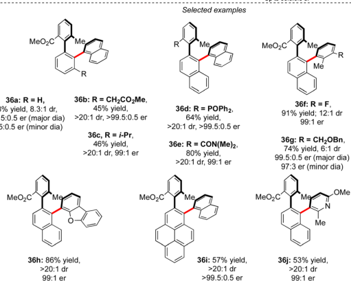
Scheme 12 Synthesis of triaryl compounds via double atroposelective direct arylation.
