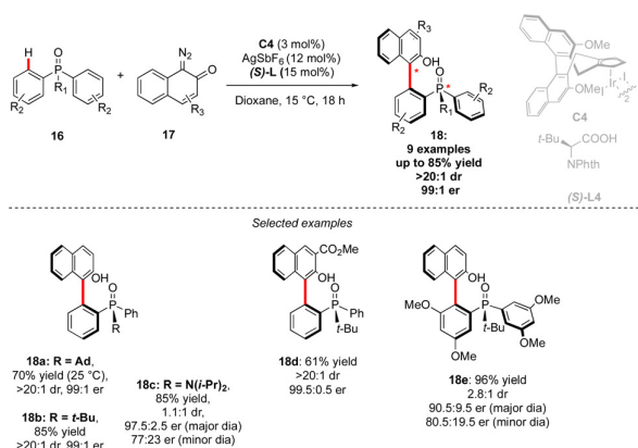
Scheme 7 C–C axial chirality + P -point chirality via desymmetrization of phosphine oxide.
