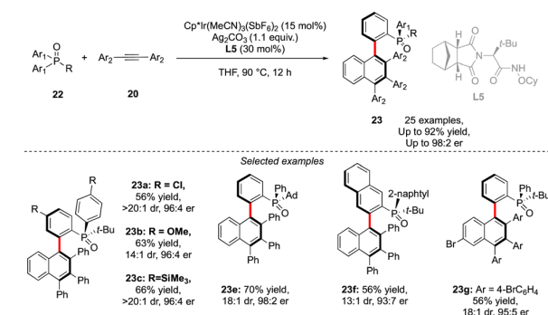
Scheme 9 Achiral Cp * Ir-complex + chiral amide ligand catalytic system to assemble scaffolds featuring C–C atropoisomerism + P -point chirality via construction of the aromatic motif.
