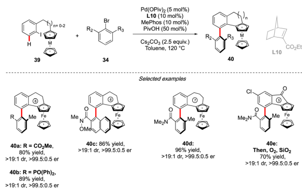
Scheme 14 Axial + planar chirality via Catellani approach.
