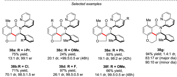
Scheme 13 Synthesis of triaryl with vicinal atropisomeric axes via intramolecular coupling.
