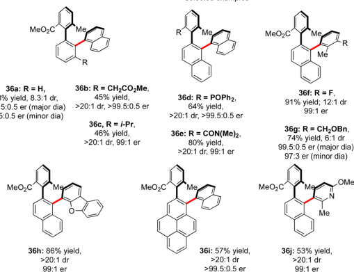
Scheme 12 Synthesis of triaryl compounds via double atroposelective direct arylation.
