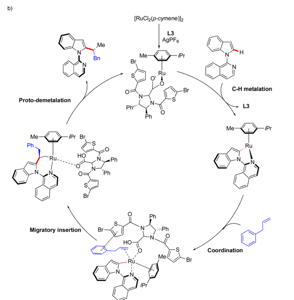
Scheme 4 Synthesis of C–N atropisomeric compounds with additional central chirality via atroposelective functionalization of a prochiral C–H substrate.
