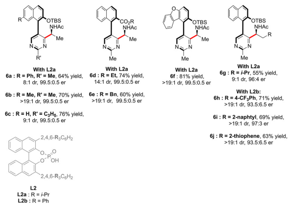
Scheme 3 Photocatalytic atroposelective Minisci-type reaction.
