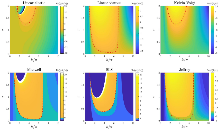
Figure 11: Effects of varying the cell traction forces. Dispersion relations corresponding to the stress-strain constitutive equations (1)-(6) for increasing cell traction forces, that is for \tau \in [0, 2] . The values of the other parameters are given by (26) and (27). White and black regions in the plots related to the linear elastic model, the Maxwell model and the SLS model correspond, respectively, to \text{Re}(\psi(k^2)) > 20 and \text{Re}(\psi(k^2)) < -20 ( i.e. a vertical asymptote is present in the dispersion relation). Red dashed lines mark contour lines where \text{Re}(\psi(k^2)) = 0 .
