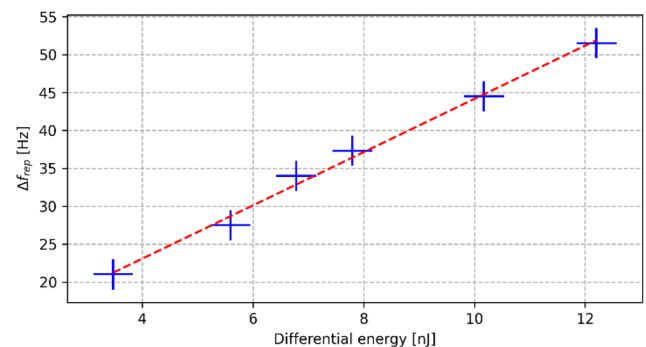
Figure 2. Repetition rate difference between the two directions as function of intra-cavity energy difference. Blue: experimental data; red: linear fit.
