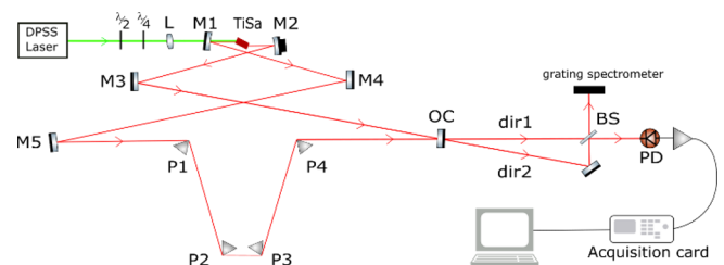
Figure 1. Home-made bidirectional Ti:Sa cavity, pumped by a 532 nm commercial cw laser (Coherent® Verdi V5). L: lens; M: mirrors; P: prisms; OC: output coupler; BS: beamsplitter; PD: photodiode. f_{rep} \approx 118 MHz.
