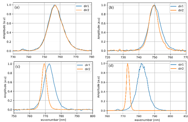
Figure 3. Normalized spectra of the two laser beams (dir1 and dir2), measured with a grating-based spectrometer for different \Delta f_{rep} values: 1.2 Hz (a), 10.4 Hz (b), 107 Hz (c), 425 Hz (d).
