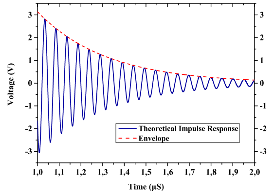
FIGURE 2. Ideal impulse response.
