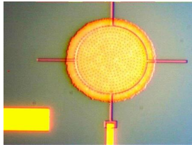
Figure 2. Optical image of the \text{Si}_3\text{N}_4 -drum, which is covered with an aluminum thin film. The drum structure is released from the silicon substrate by a dry etching process, which is performed through those small holes patterned circularly on the top of the drum by using electron beam lithography.
