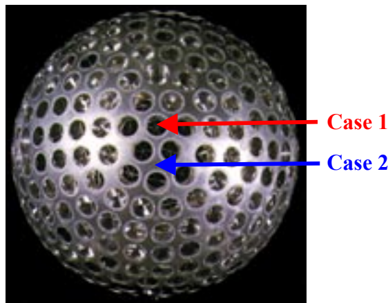
Figure 6: Difference of the mean impact point position on the LAGEOS satellite surface between the two extreme cases. In the case 1, the mean impact point corresponds to a CCR face. In the case 2, the impact point meets the satellite surface among 3 distinct CCRs.
