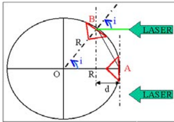
Figure 5: Geometrical parameters used for the computation.
