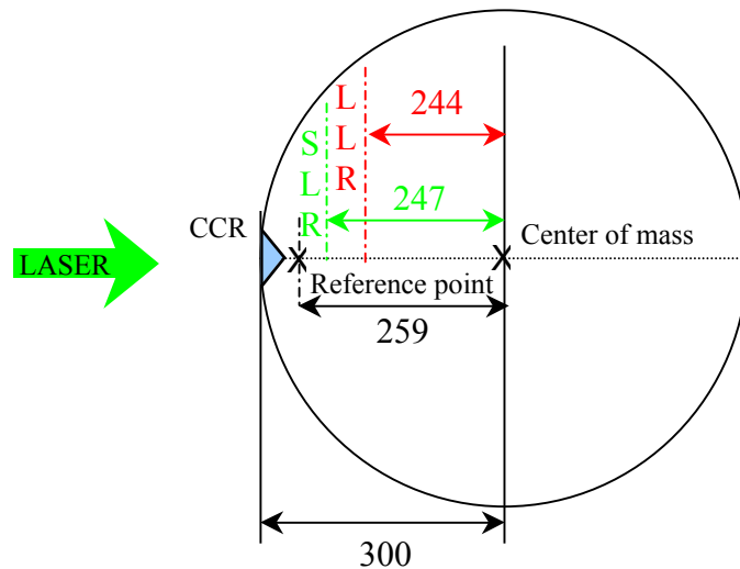
Figure 10: Center of mass corrections in millimeters for the different Grasse SLR and LLR stations for the LAGEOS satellites.
