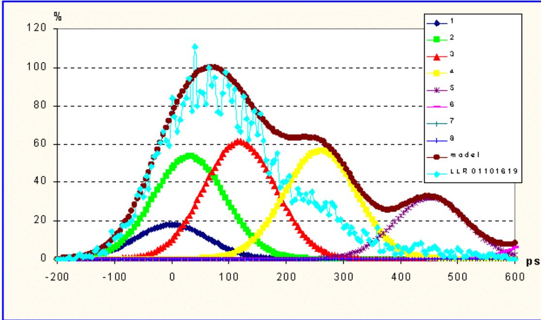
Figure 7: LAGEOS –2 pass of the 16 th October 2001. The contribution of each row of CCRs up to the 8 th and the final model obtained with the convolution of each row contribution (in brown) are represented. The cyan curve corresponds to the real raw data observed by the OCA LLR station.
