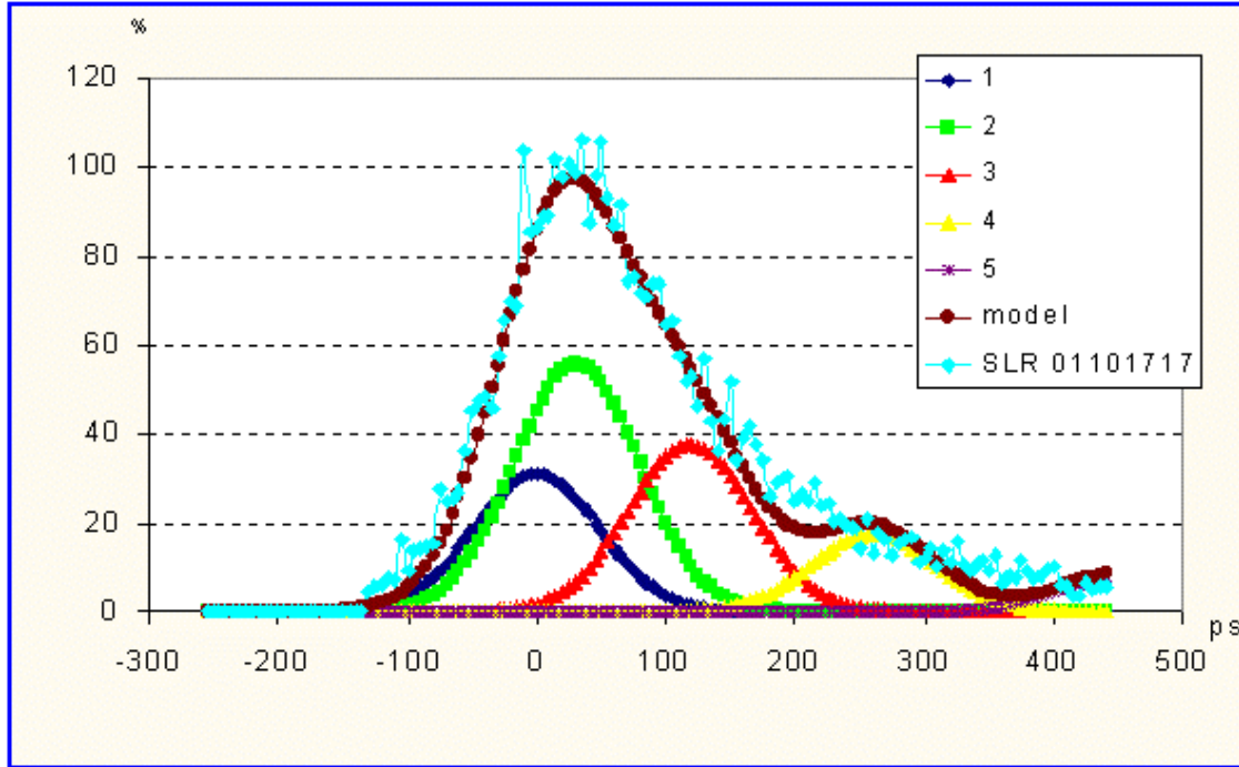
Figure 9: LAGEOS -2 pass (17 th October 2001). Comparison between the OCA SLR raw data (cyan) and the computed model (brown). The contribution of each row up to the 5 th to the satellite response are also indicated.
