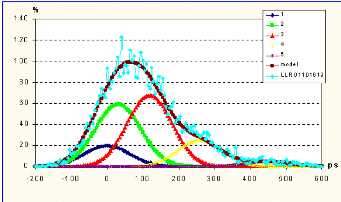
Figure 8: Comparison between the LAGEOS –2 LLR raw data (pass of the 16 th October 2001) and the satellite response model with the attenuation factors. The contribution of each row up to the 5 th are also indicated.
