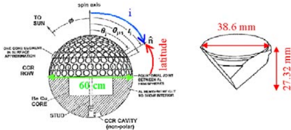
Figure 3: Repartition and dimensions of the CCRs on the LAGEOS satellite (Slabinski, 1997).
