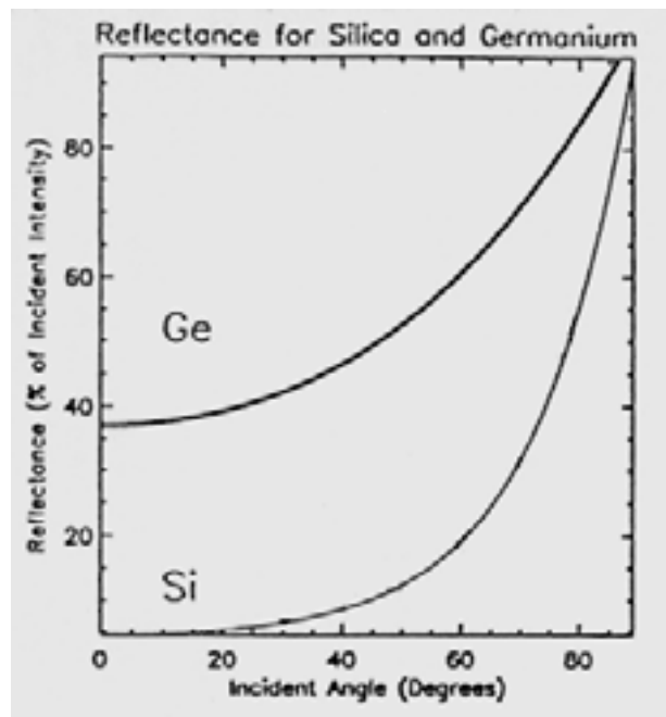
Figure 4: LAGEOS CCR reflectance curve (Avizonis, 1997).
