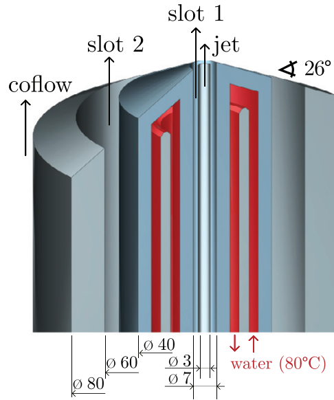
Figure 1: MRB burner geometry, from [29].
