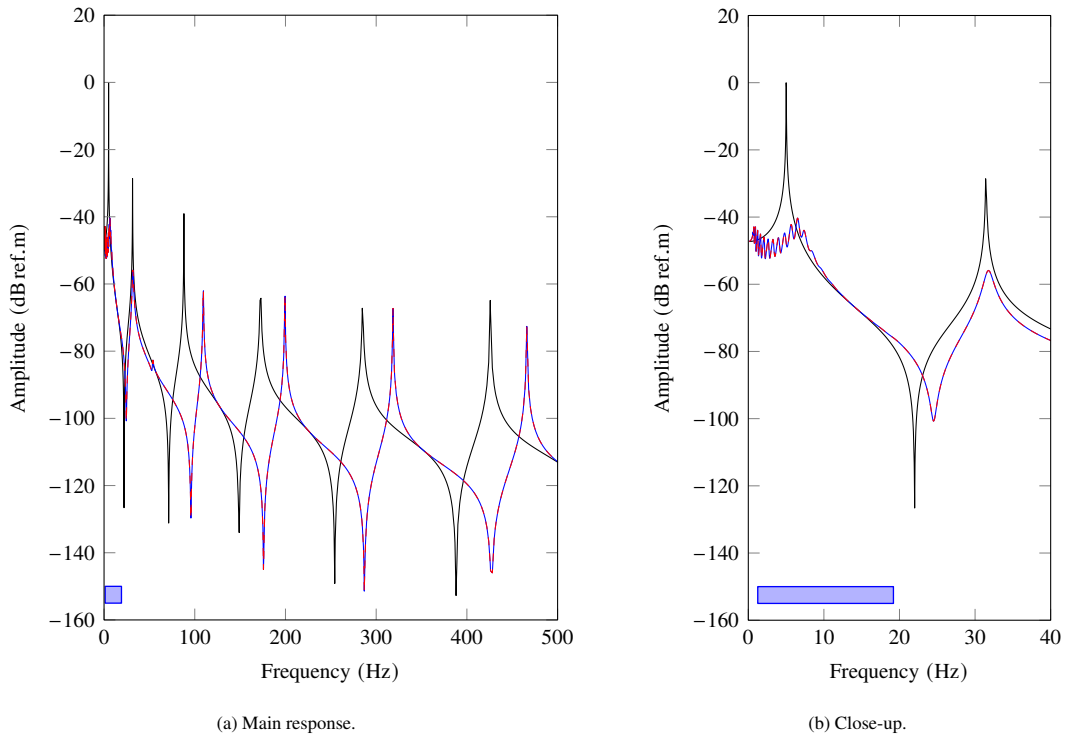
Figure 8: FRF of the pseudo-located approach with an ABH length of 3000mm. (—): plant, (- -): reference VABH, and (- . -): VABH with PZTs.
