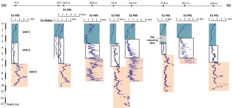
Figure 5: Geotechnical cross-section of the eastern edge of paleomeander (site E1)
