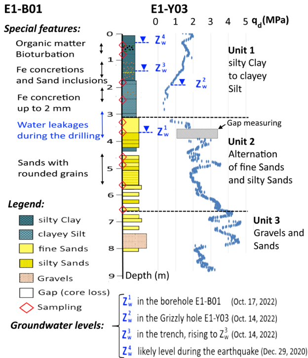
Figure 3: Stratigraphy in the first 9 meters
