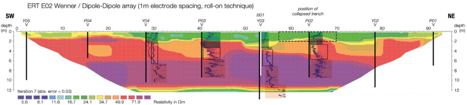
Figure 6: Electrical Resistivity Tomography (ERT) profile (E02) with 1 meter spacing measured in a dipole-dipole and Wenner array (roll-on technique). Some data from the DCPT tests are included to show the correlation between geotechnical and geophysical data. Black solid lines: reached depth with the DCPT tests; white solid line: reached depth for core-borehole B01; dashed rectangle: extent of the collapsed trench.
