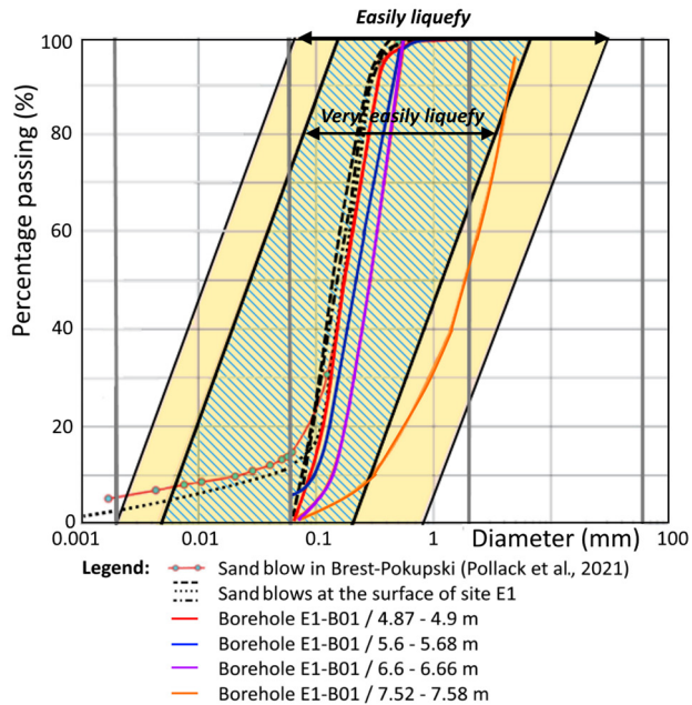
Figure 4. Site E1 - Cumulative particle size - plots for sands
