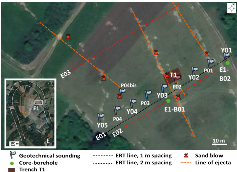
Figure 2. Location of field investigations at E1 site
