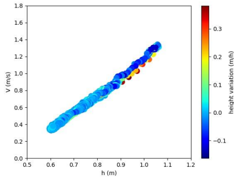
Figure 6. Flow characterization in March 2019: velocity as a function of water level.
