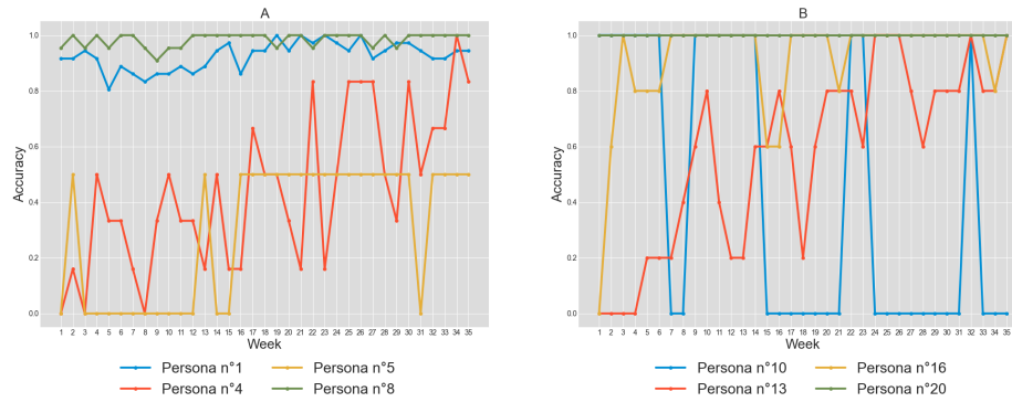
Fig. 4. Accuracy evolution of personas of logs (A) and no_logs (B) subdatasets.
