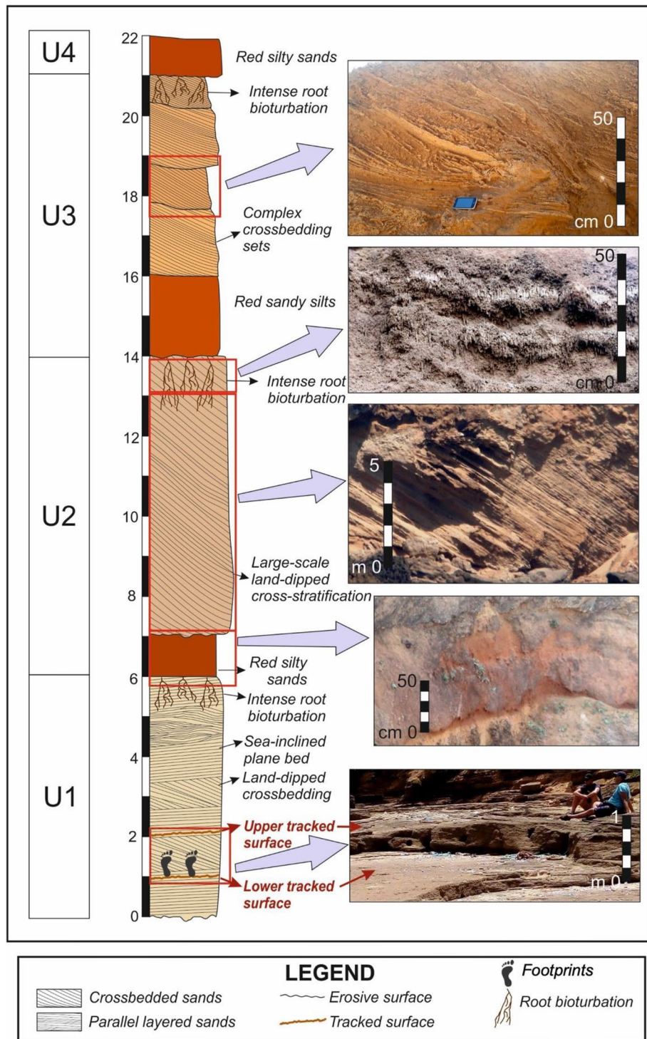
Figure 2. Sedimentary log of Larache site cliff. The right border of the sediment bodies in the log indicates the relative changes in average grain size. The colours of the bodies represent the approximate natural colour of the sediments. Pictures illustrate the aspects of some of the sediment bodies.
