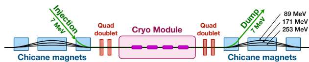
Figure 2: Common Section layout of 250 MeV version.
