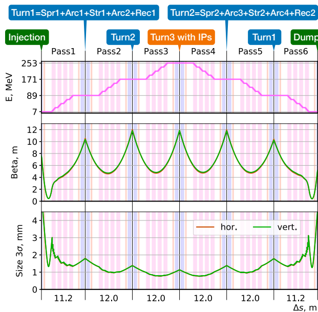
Figure 3: Beam energy, beta function and size during six passes through the Common Section.
