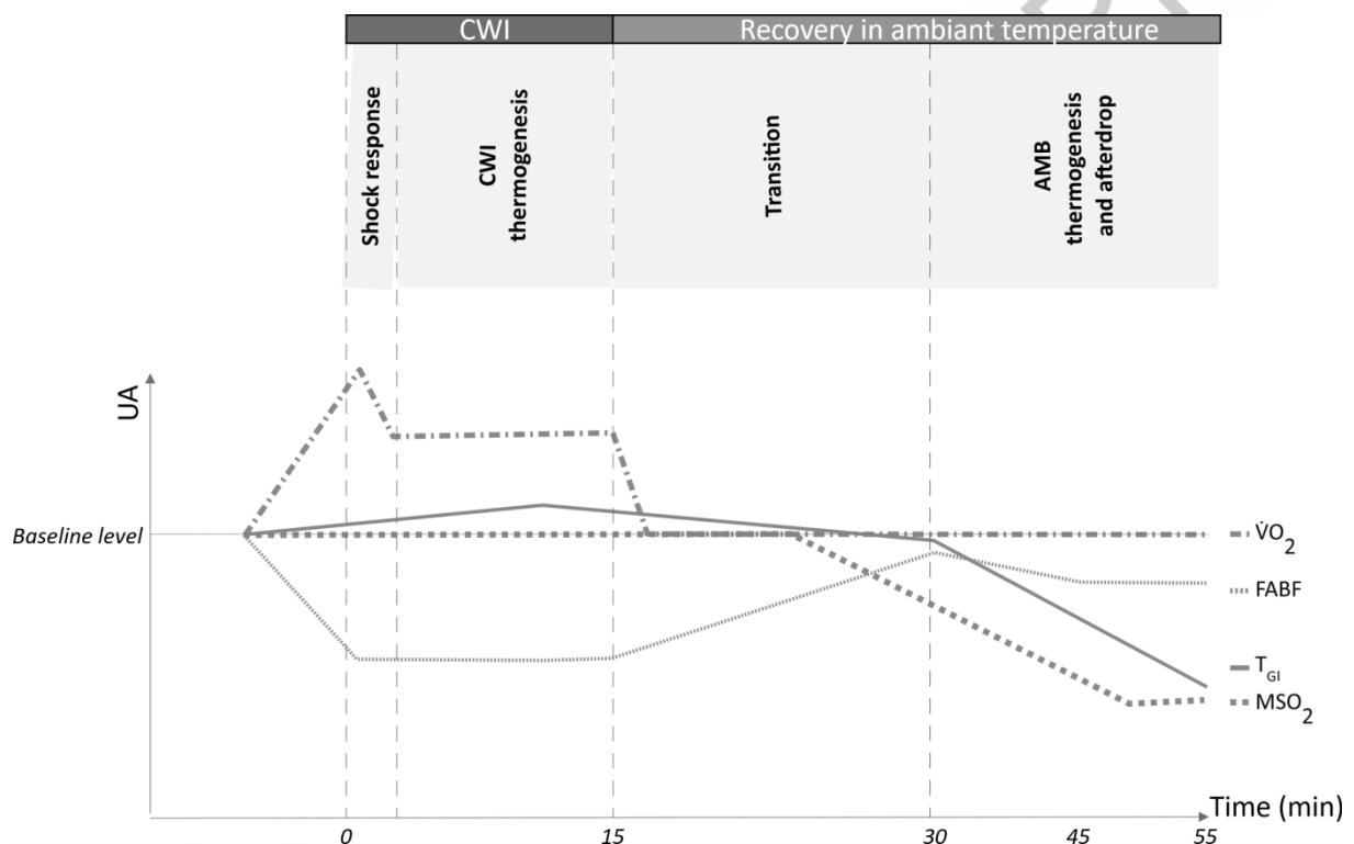
Figure 6: schematic evolution of oxygen consumption ( \dot{V}O_2 ), gastrointestinal temperature ( T_{GI} ), muscle O_2 saturation ( MSO_2 ) and arterial blood flow (FABF) during the CWI and the rewarming.
