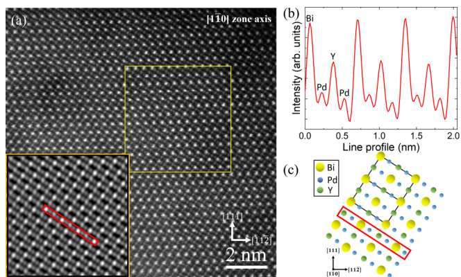
FIG. 11. (a) Raw STEM-HAADF image of \text{PdYBi} . The inset is a processed image of the yellow frame in the raw image. The better signal-to-noise ratio allows us to clearly distinguish the atomic columns and their intensities. (b) Intensity line profile performed on the inset red box area. (c) Sketch of the observed column pattern.
