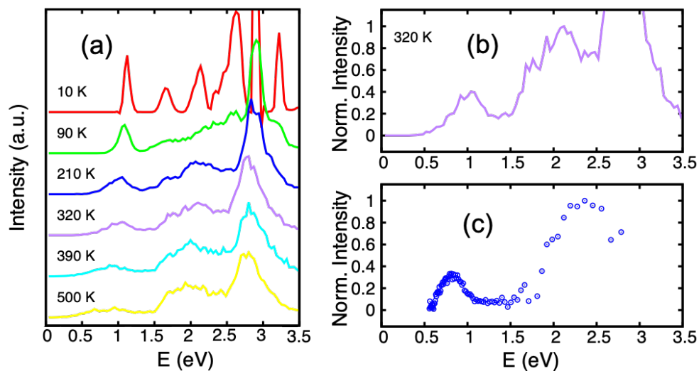
Fig. 7 Experimental action spectrum (photodissociation-c) of \text{Py}_2^+ compared with photoabsorption spectra computed for various temperatures (a-b, DFTB-EXCI). Adapted from Ref. 221 with permission from the PCCP Owner Societies. Copyright 2021.
