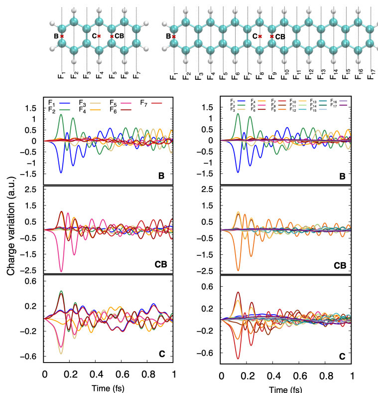
Fig. 3 Ultrafast charge evolution for anthracene and octacene after collision with a 100 keV proton impacting the center of a central aromatic ring (C) or an central (CB) or border (B) bond.
