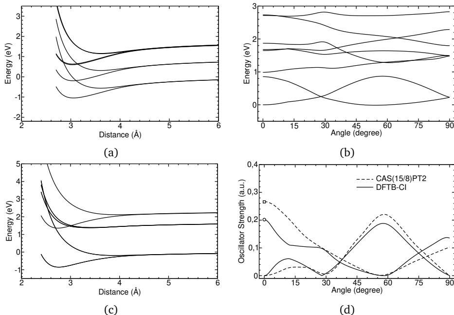
Fig. 1 DFTB-EXCI energetic profiles for ground and excited states for cationic dimers of pyrene (a,b) and benzene (c) in superimposed approach path (a,c) or following a twisting mode (b). Oscillator strengths for the two first excitations along this path are also reported together with CASPT2 results (d). Adapted from Ref. 172 with permission from the PCCP Owner Societies. Copyright 2016.
