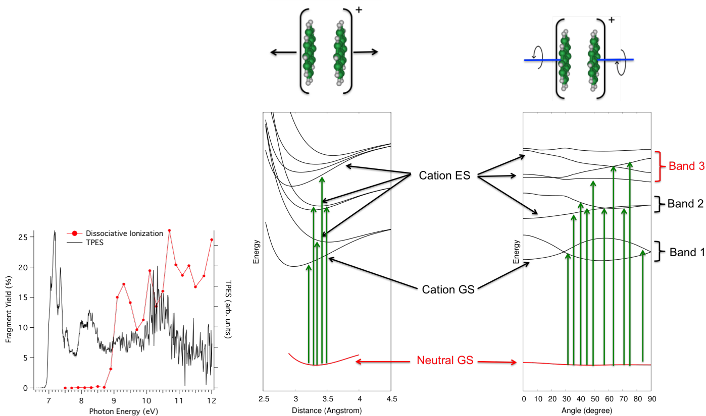
Fig. 8 Left : Photoionisation (black) and photoionisation+dissociation (red) spectra for \text{Py}_2 recorded at SOLEIL synchrotron apparatus. Right : computed electronic ground states of \text{Py}_2 and \text{Py}_2^+ and first electronic excited states of \text{Py}_2^+ according to dissociative breathing mode (left) and non-dissociative twist mode (right). Adapted from Ref. 222 with permission from the PCCP Owner Societies. Copyright 2023.
