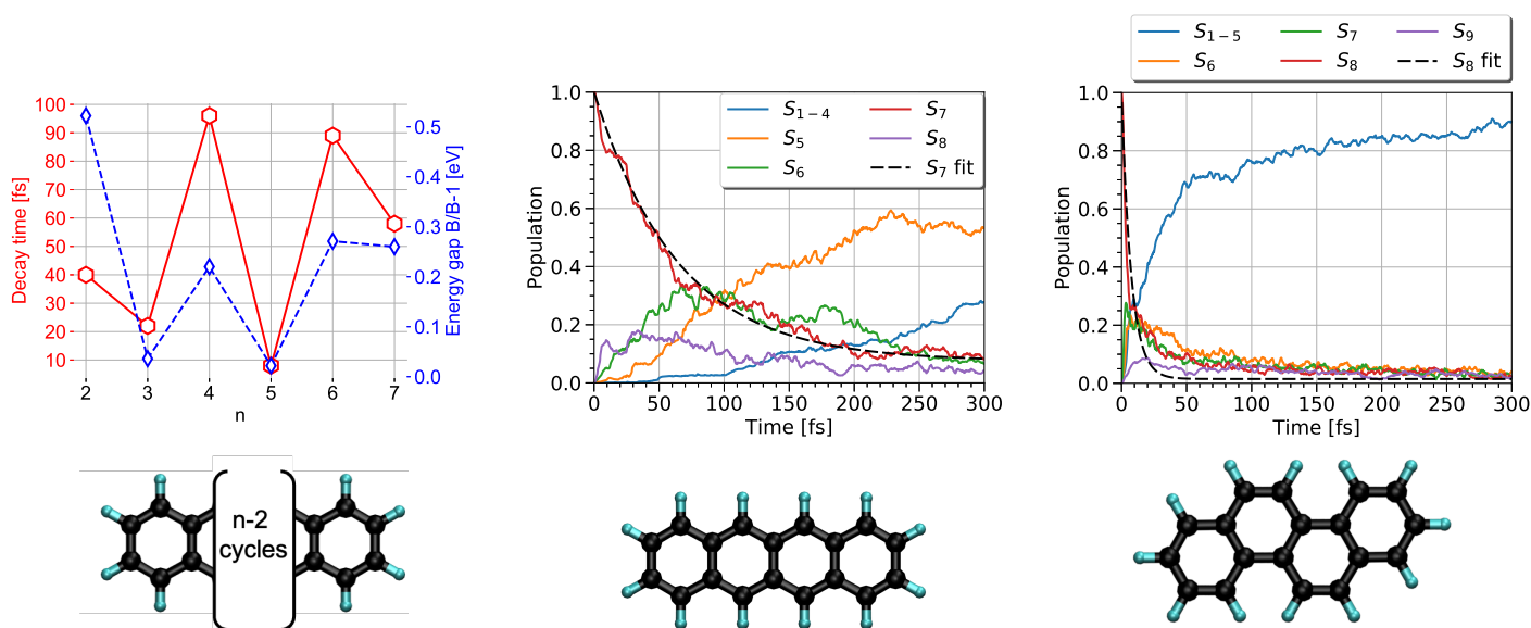
Fig. 5 Left : correlation between the electronic relaxation timescales from the brightest state and energy gap below the latter and the state just below for polyacenes ( n is the number of aromatic cycles). Time evolution of the states population for tetracene (middle) and chrysene (right) molecules. Left : adapted from Ref. 191 with permission from the PCCP Owner Societies. Right : adapted from Ref. 216 with acknowledgements of AIP. Copyright 2020.
