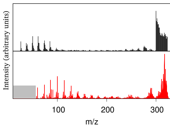
Fig. 2 Experimental (black) and calculated (red) mass spectrum in arbitrary units of a coronene heated by successive hydrogenations ( m/z=300 : bare coronene; m/z>300 : hydrogenated coronene; m/z between 275 and 285: loss of C_2H_n fragments). Adapted from Ref. 201 with permission from the PCCP Owner Societies. Copyright 2018.
