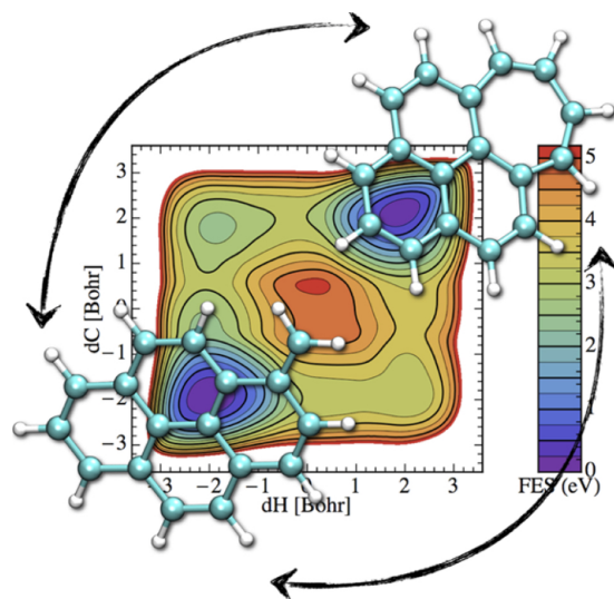
Fig. 6 Free energy map for isomerisation of the methylene pyrene cation. Reprinted with permission from Ref. 220 . Copyright 2015 American Chemical Society.
